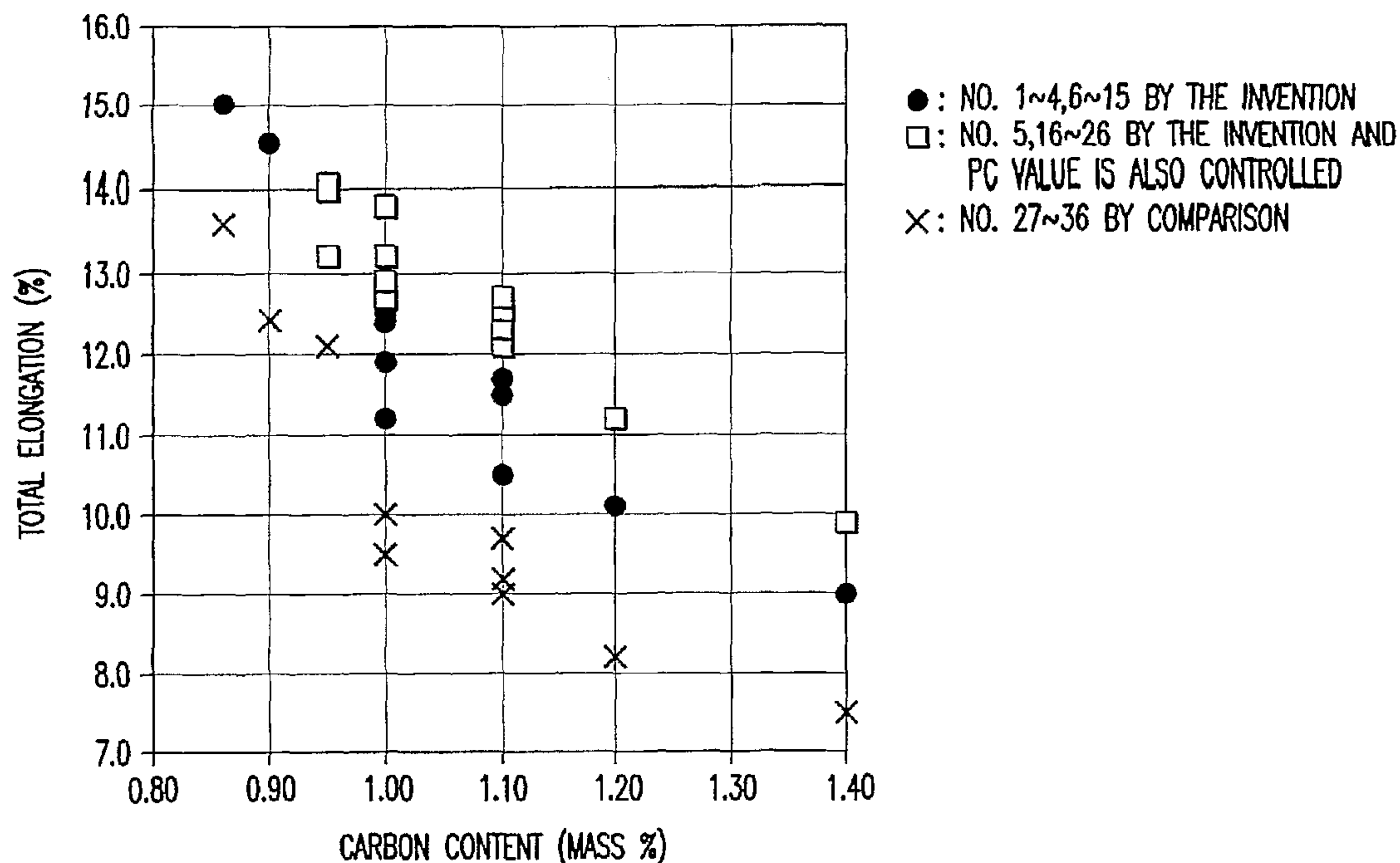
RELATIONSHIP BETWEEN THE CARBON CONTENT AND THE TOTAL ELONGATION VALUE OF THE RAIL
