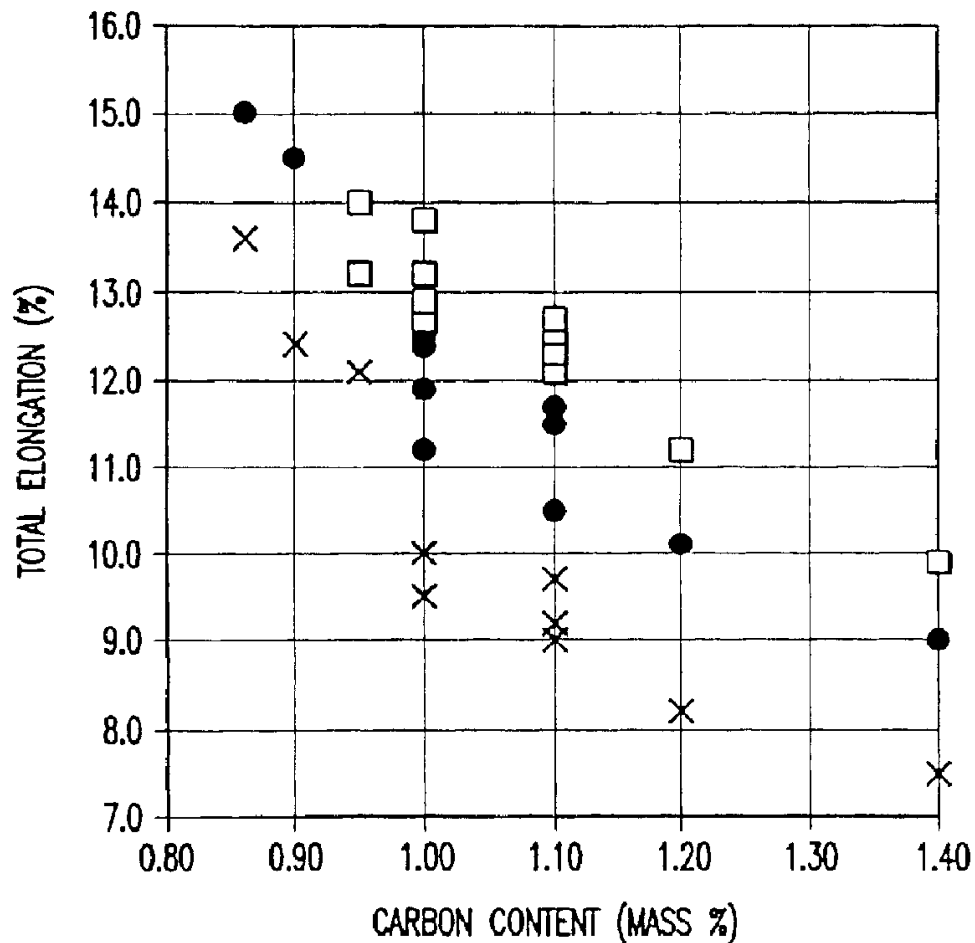
RELATIONSHIP BETWEEN THE CARBON CONTENT AND THE TOTAL ELONGATION VALUE OF THE RAIL
