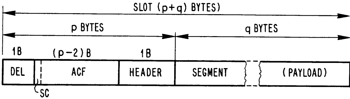
FIG. 3 SLOT STRUCTURE
