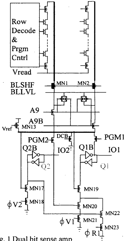
Fig. 1 Dual bit sense amp
