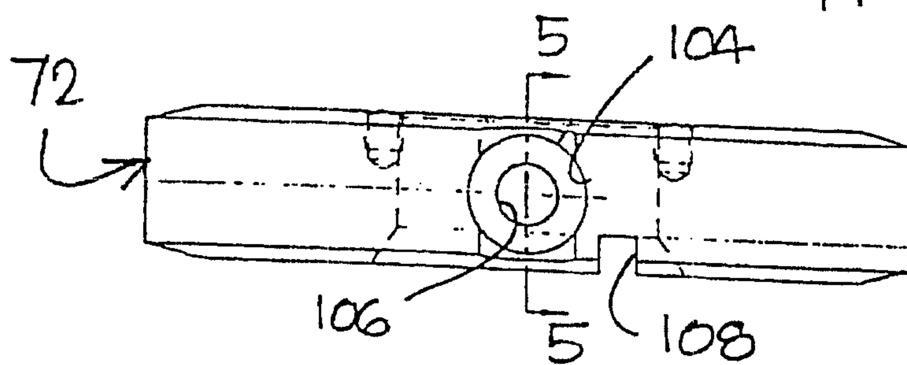
OUTSIDE VIEW OF TYP. WEDGE
