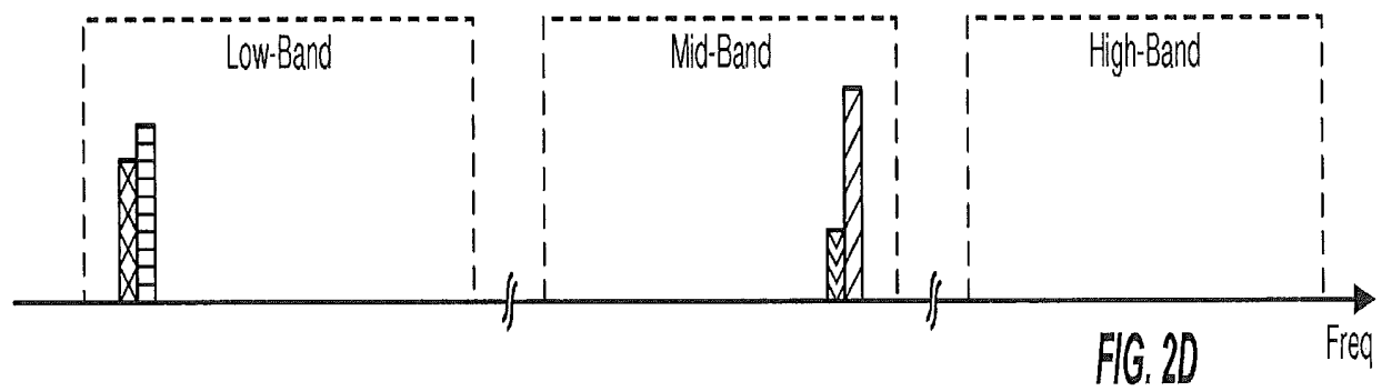
Inter-Band Carrier Aggregation in Different Band Groups
