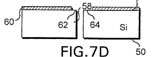
STEP 4. FORM NITRIDE PATTERN MASK
