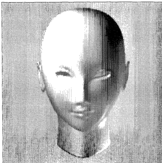
implicit function (mesh: 90 \times 90 \times 90 )
