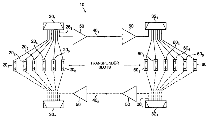
RECONFIGURABLE MUX/DEMUX TO ENABLE WAVELENGTH INDEPENDENT TRANSPONDER SLOTS THAT CAN BE WIRED WITH FIXED OPTICAL CONNECTIONS AND SEND/RECEIVE ANY λ
