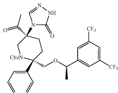
Compound 53a
