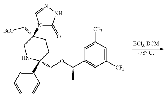
Compound 35d
