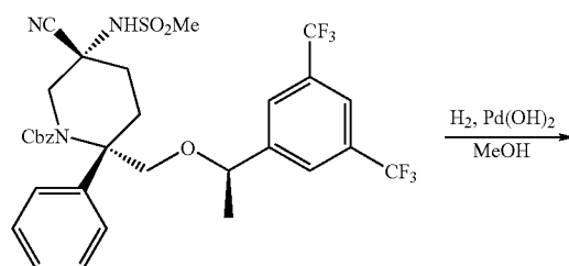
Compound 37a
