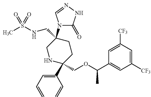
Compound 15
