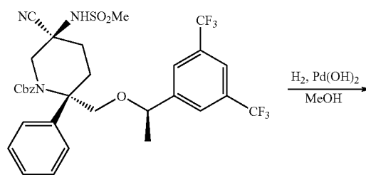
Compound 36a
