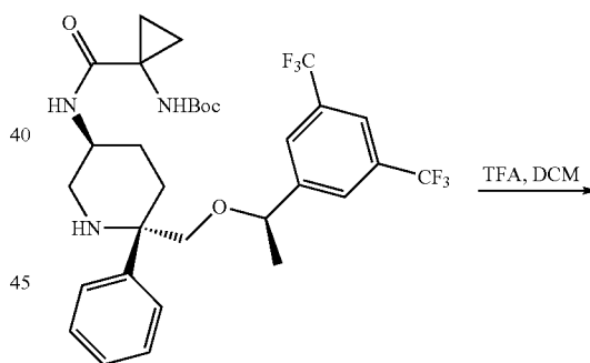
Compound 43a
