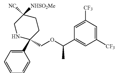
Compound 36
