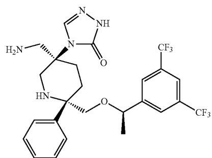
Compound 15b
