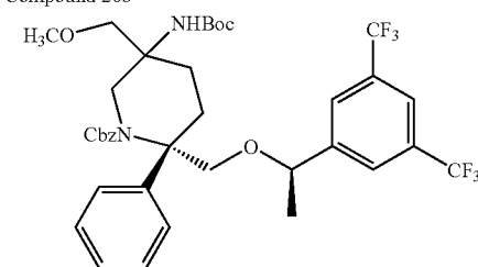
Compound 26c
