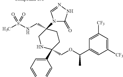
Compound 15
