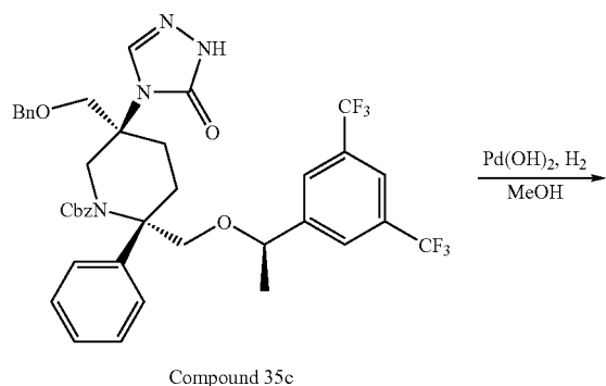
Compound 35c
