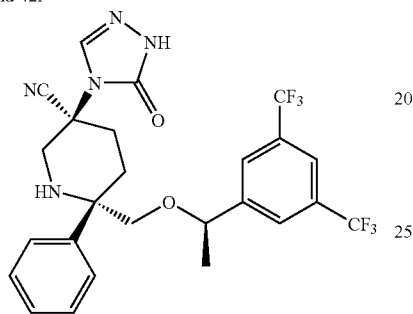
Compound 42
