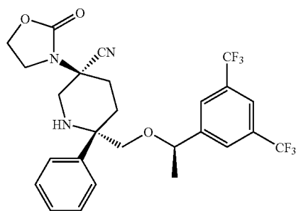
Compound 2
