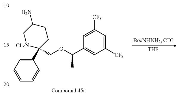
Compound 45a
