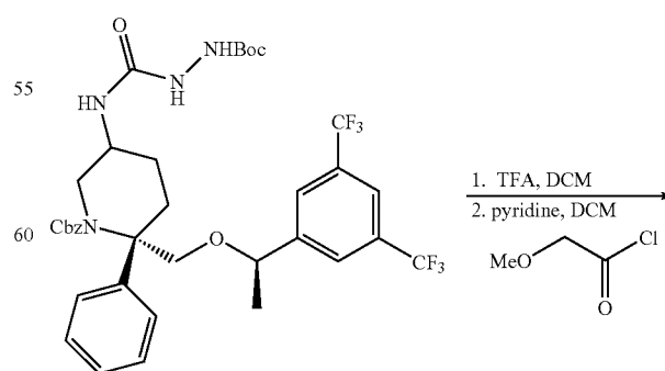
Compound 45b
