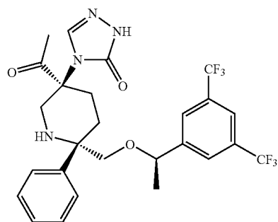
Compound 53
