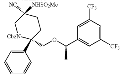
Compound 36a
