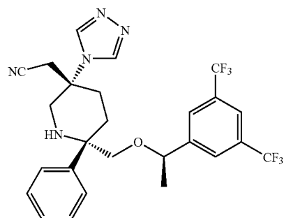
Compound 5d
