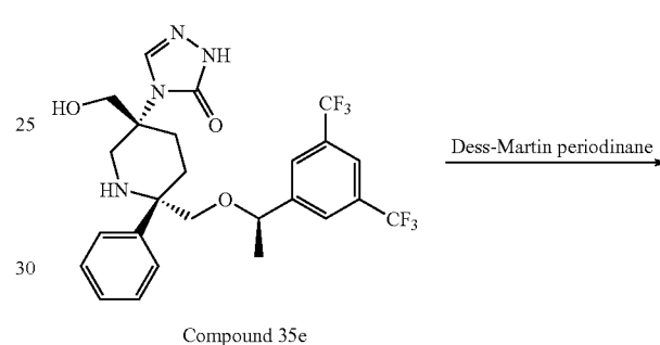
Compound 35e
