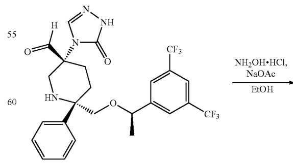
Compound 35f
