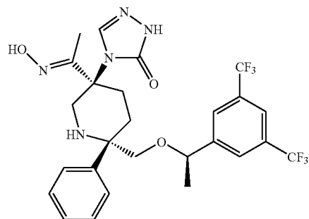
Compound 54
