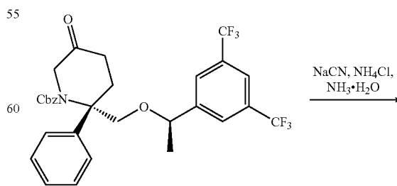
Compound 41a
