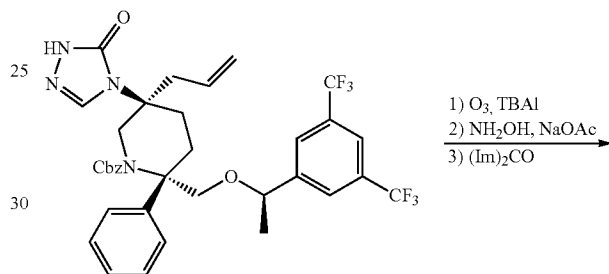
31g
