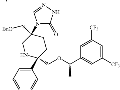
Compound 35d
