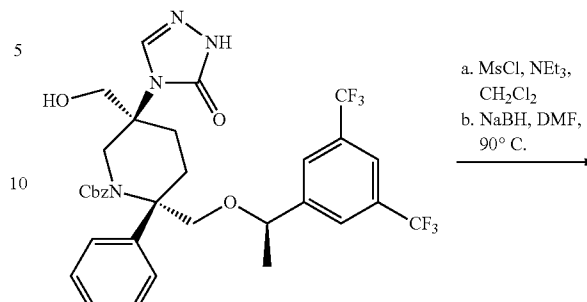
Compound 23h
