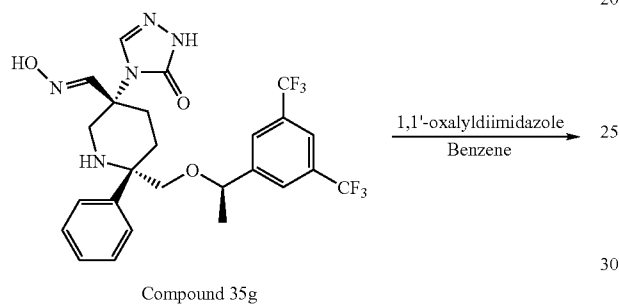
Compound 35g
