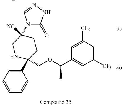
Compound 35g
