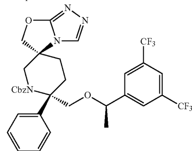
Compound 56a
