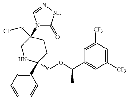
Compound 56
