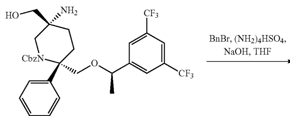
Compound 35a
