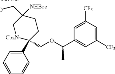
Compound 26b
