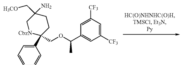
Compound 26a
