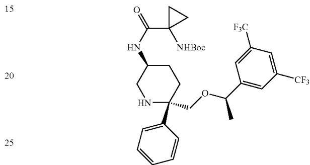
Compound 43a
