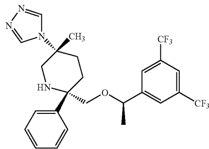
Compound 6
