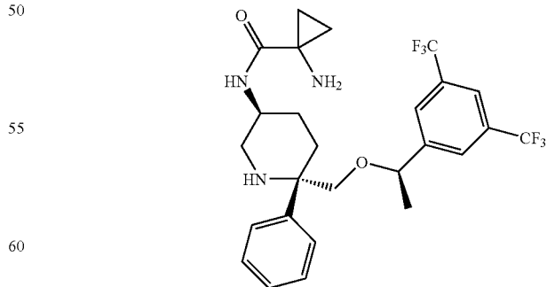
Compound 43b
