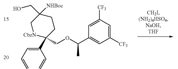
Compound 26b
