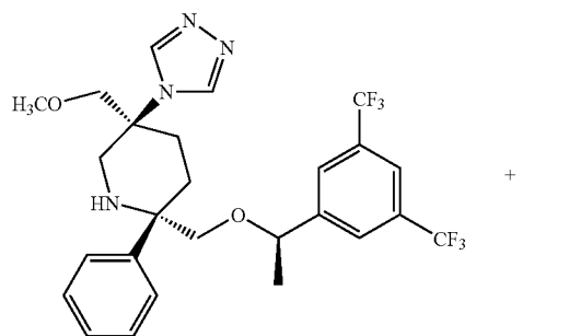
Compound 13
