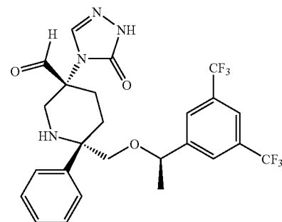
Compound 35f
