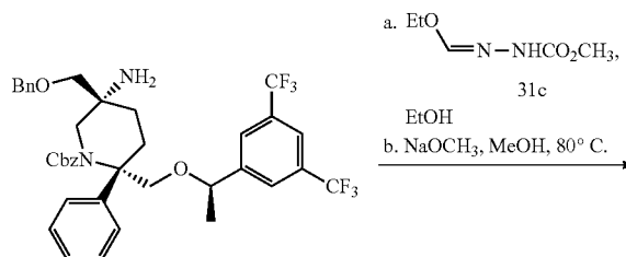
Compound 35b
