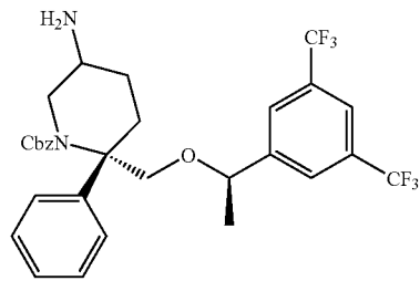
Compound 45a
