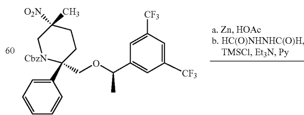
Compound 6a
