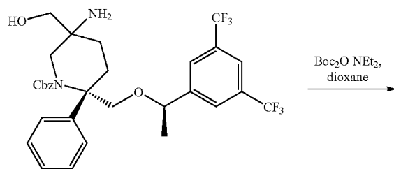
Compound 26a
