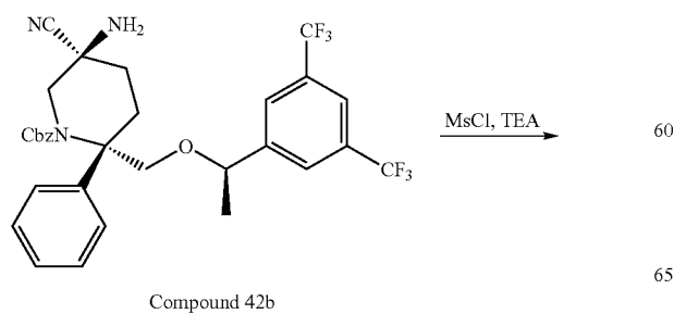
Compound 42b
