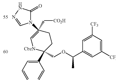
31h
