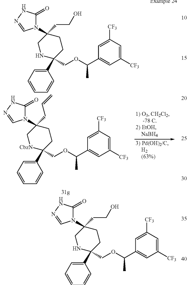
Example 24
