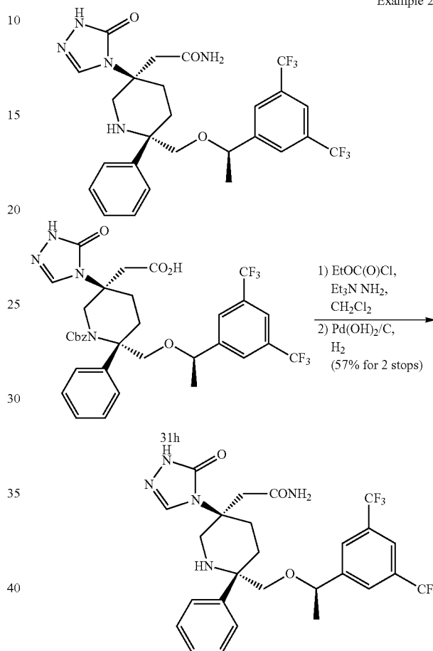
Example 29
