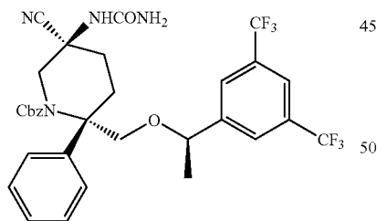
Compound 41a
