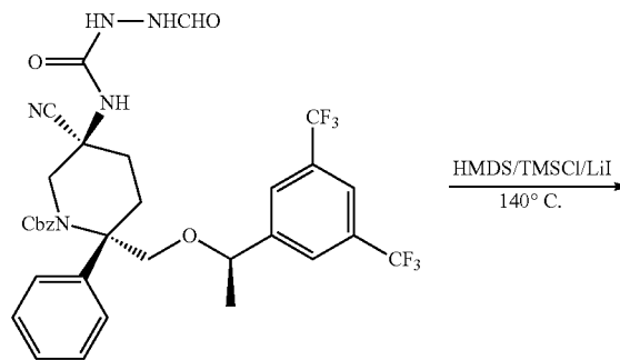
Compound 42d
