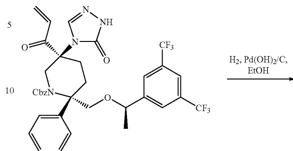
Compound 19a
