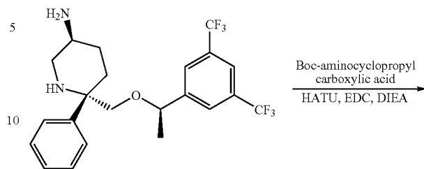
Compound 44b
