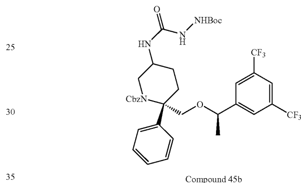
Compound 45b
