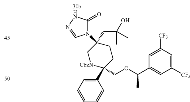
11a
