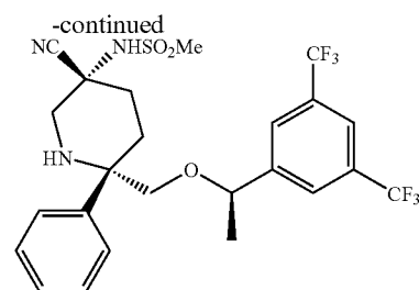
Compound 37
