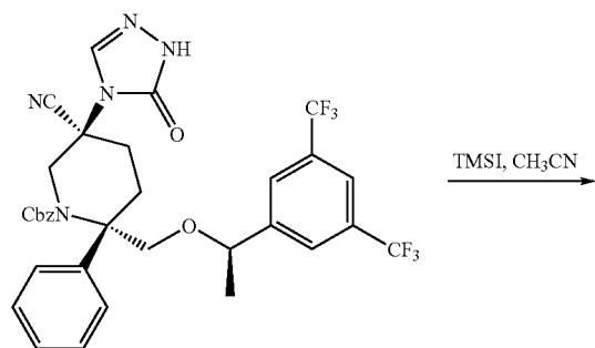
Compound 42i
