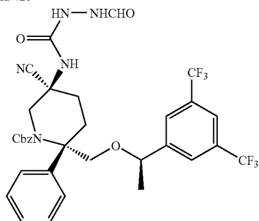
Compound 42d
