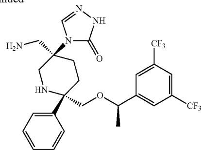
Compound 15b
