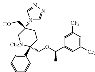
Compound 12a
