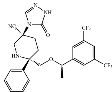
Compound 42
