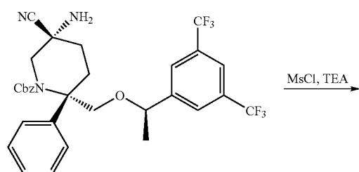
Compound 42b
