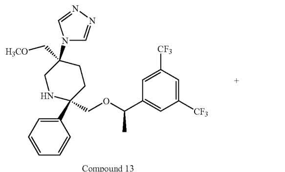
Compound 13
