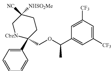
Compound 37a
