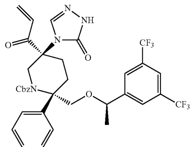
Compound 19a
