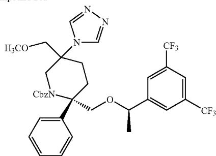
Compound 14a
