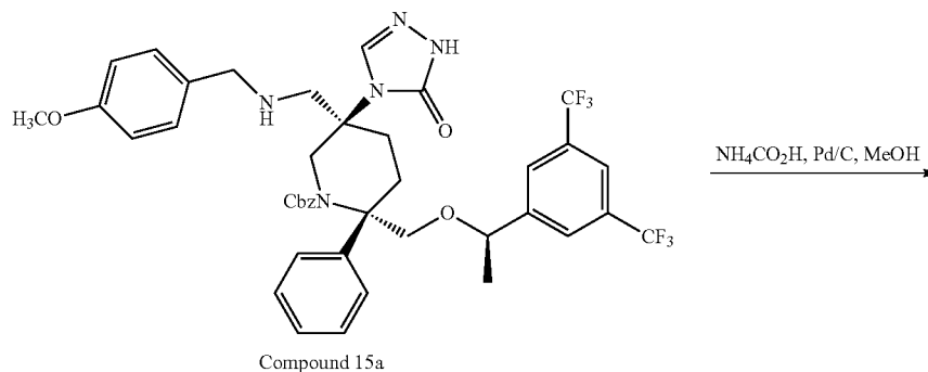
Compound 15a
