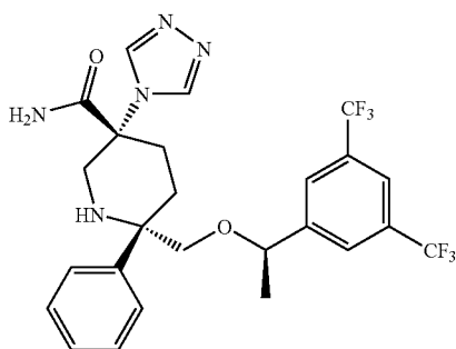
Compound 10
