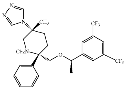
Compound 6b
