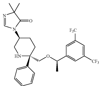
Compound 28
