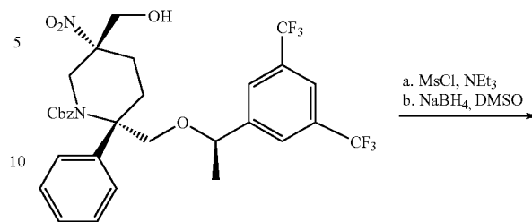
Compound 23d
