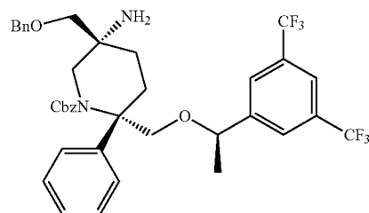
Compound 35b
