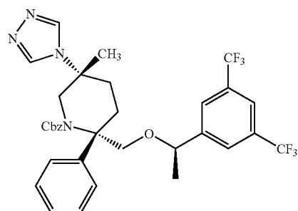
Compound 6b
