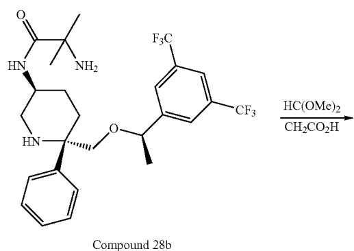
Compound 28b
