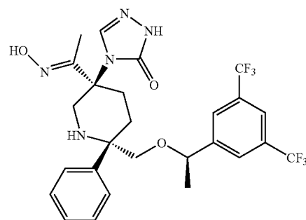
Compound 54
