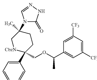
Compound 57a
