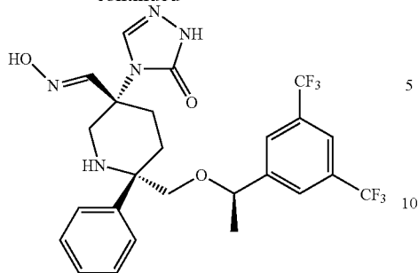
Compound 35g
