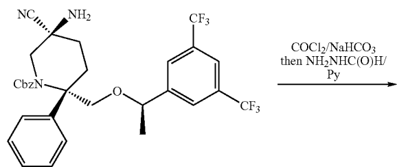
Compound 42b
