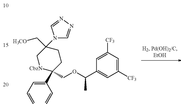
Compound 14a
