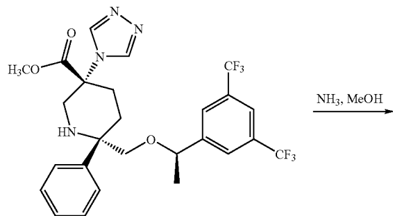
Compound 8
