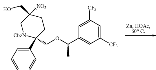
Compound 23d
