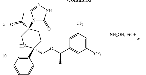
Compound 53
