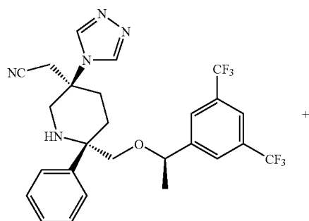
Compound 5
