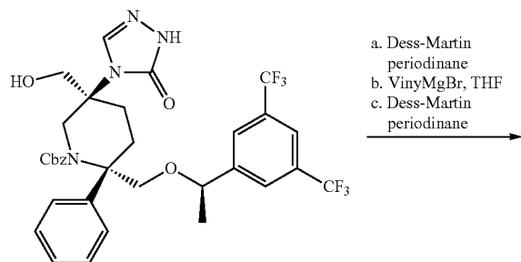
Compound 23h
