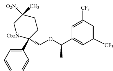
Compound 6a
