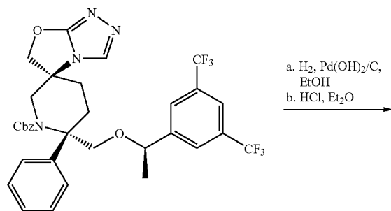
Compound 56a
