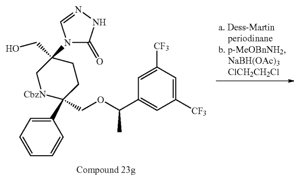
Compound 23g
