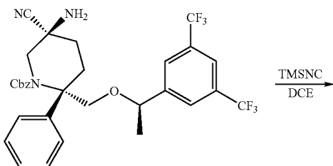
Compound 42b
