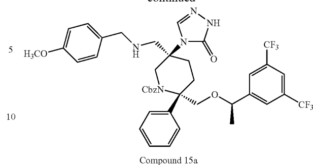
Compound 15a
