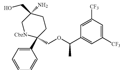
Compound 35a
