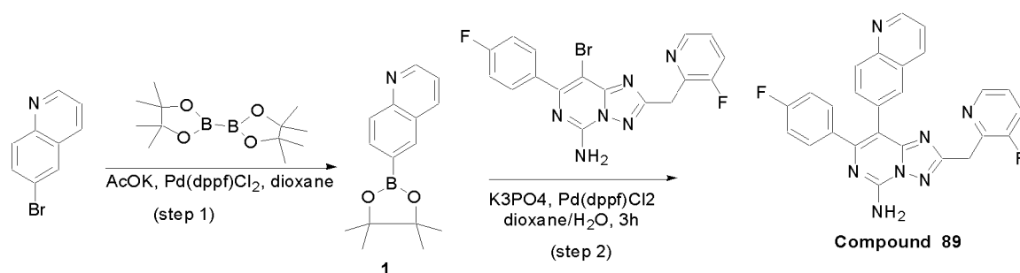
SCHEME 43
