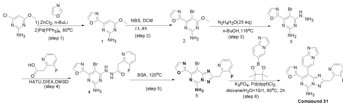
SCHEME 19
