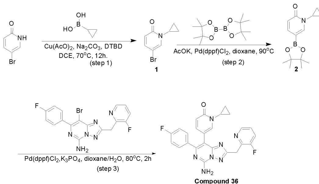
SCHEME 23
