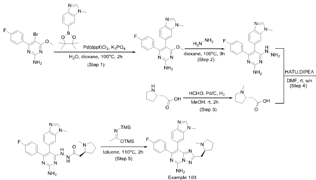
SCHEME 47
