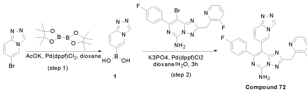
SCHEME 41
