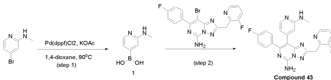
SCHEME 27
