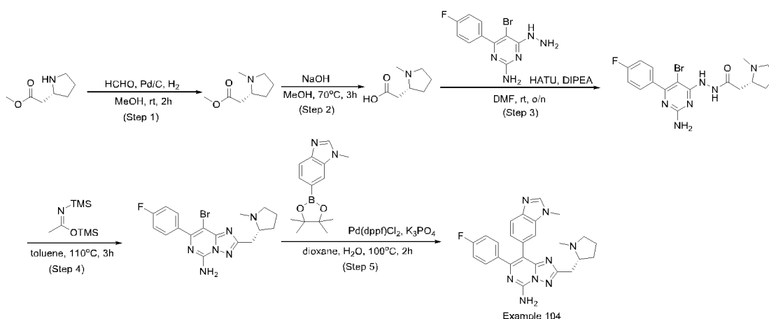
SCHEME 48
