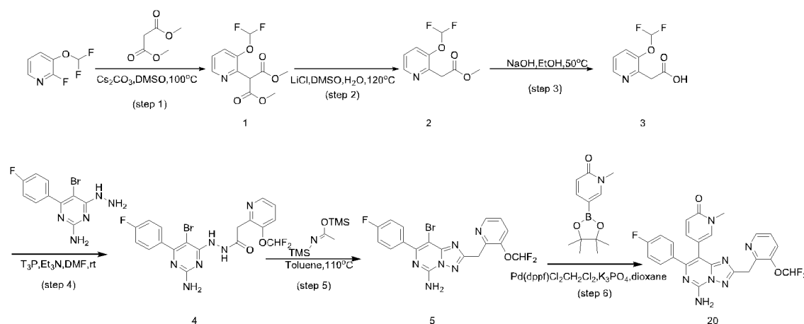
SCHEME 11
