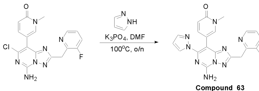
SCHEME 35
