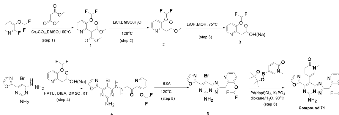
SCHEME 40
