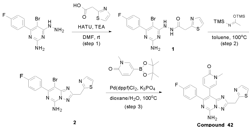
SCHEME 26
