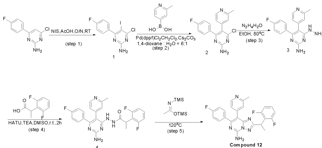
SCHEME 6
