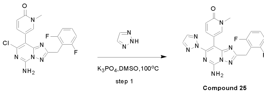
SCHEME 16
