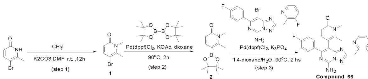
SCHEME 37
