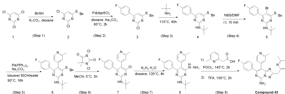
SCHEME 28
