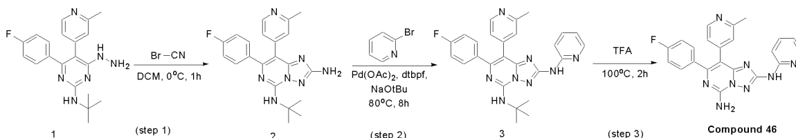
SCHEME 29
