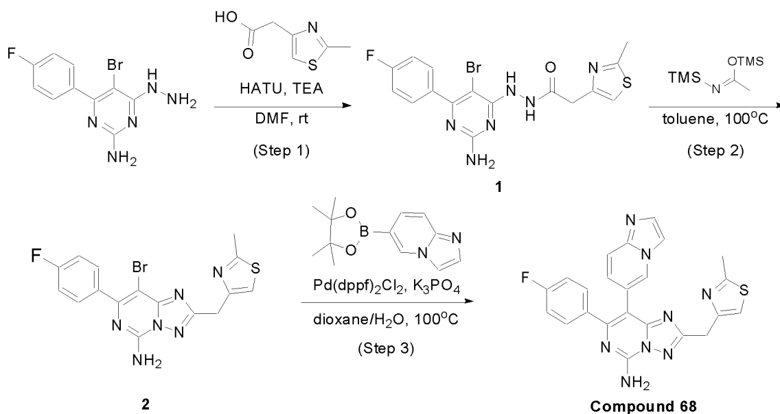
SCHEME 39
