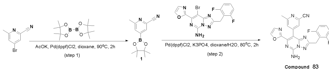
SCHEME 42
