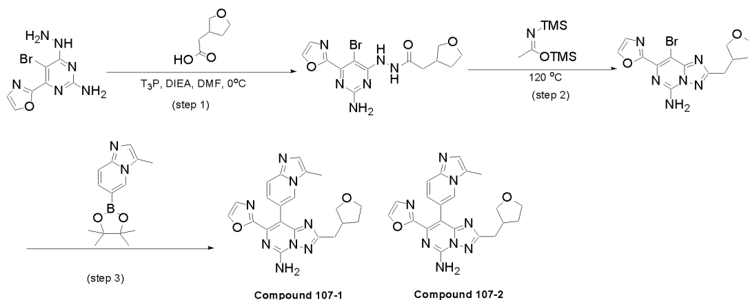
SCHEME 50
