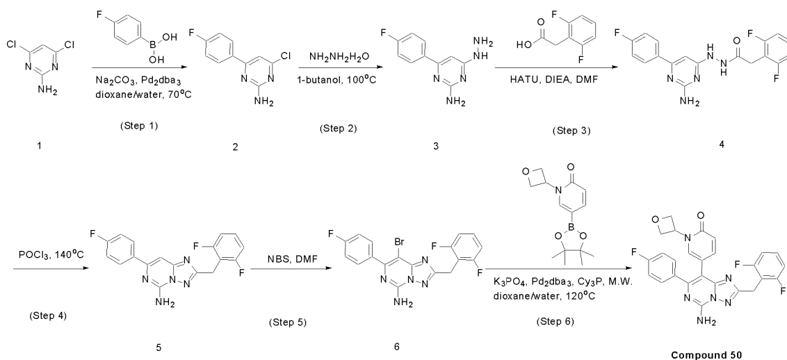
SCHEME 31
