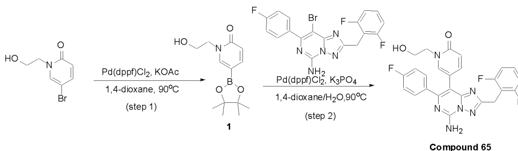
SCHEME 36
