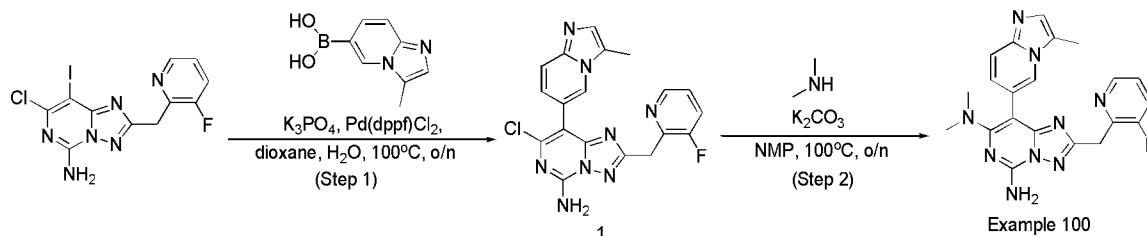
SCHEME 46
