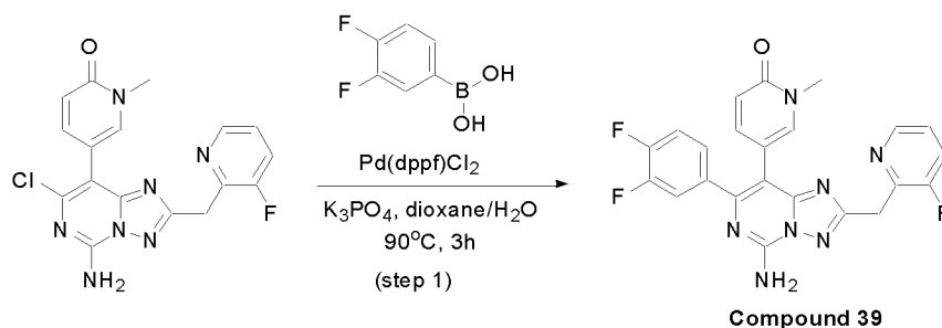
SCHEME 25
