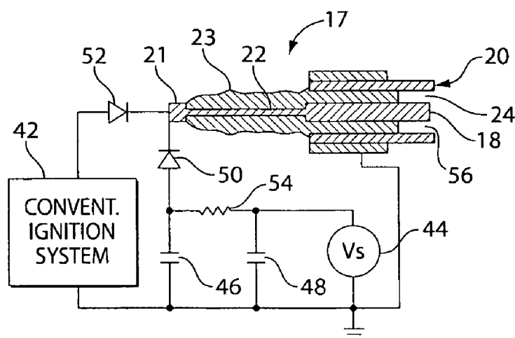
Fig. 2 (Prior Art)
