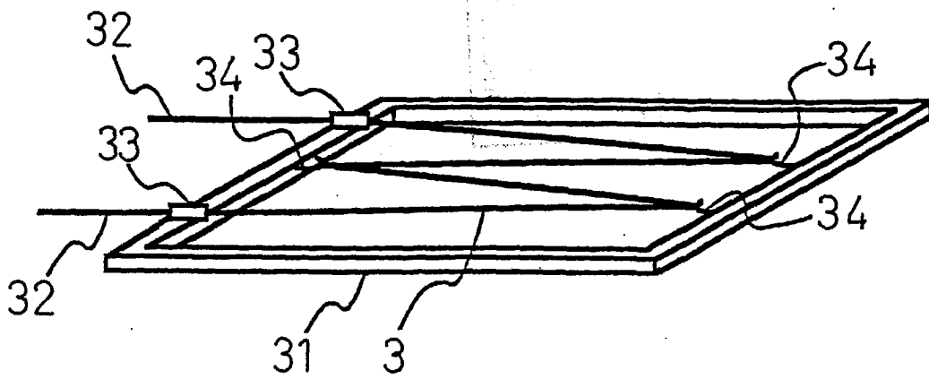
FIG. 8 (prior art)
