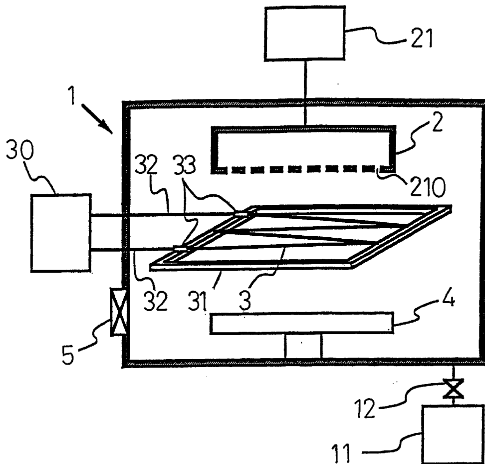
FIG. 7 (prior art)
