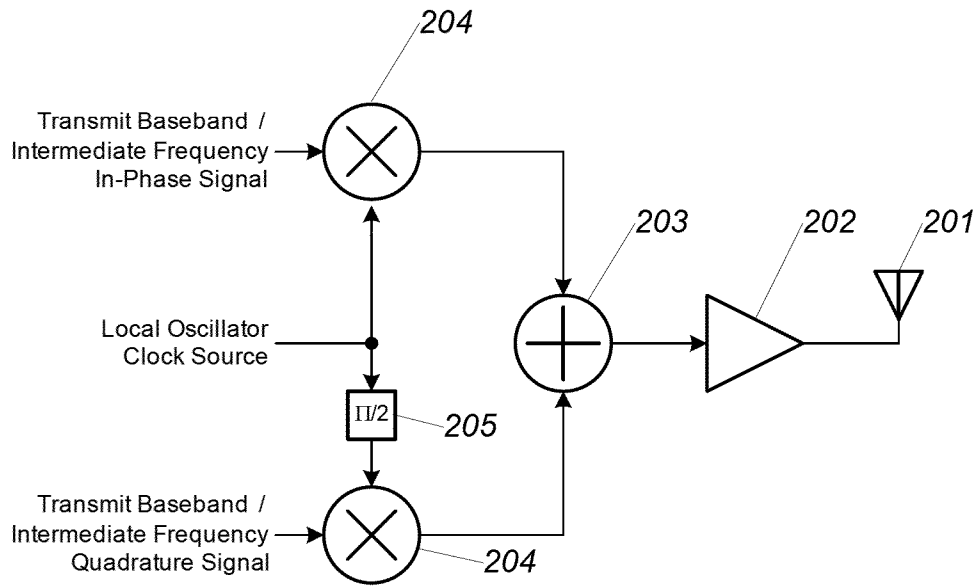
Figure 2 (PRIOR ART)
