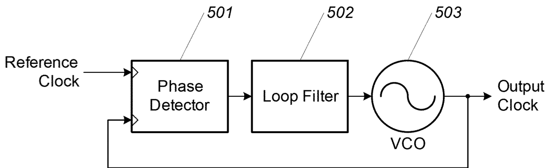
Figure 5 (PRIOR ART)
