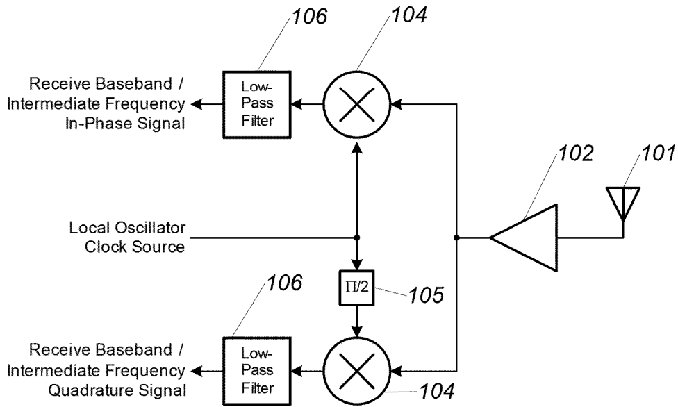
Figure 1 (PRIOR ART)
