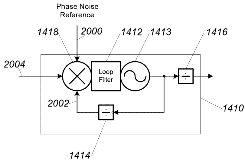
Figure 14A
