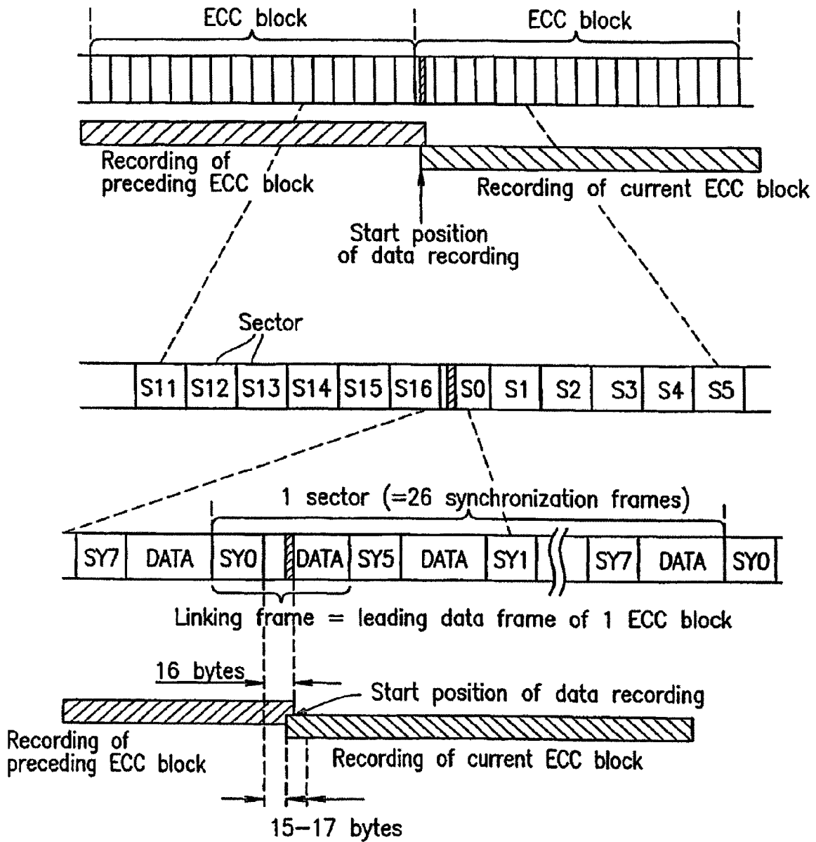
FIG. 44 CONVENTIONAL ART
