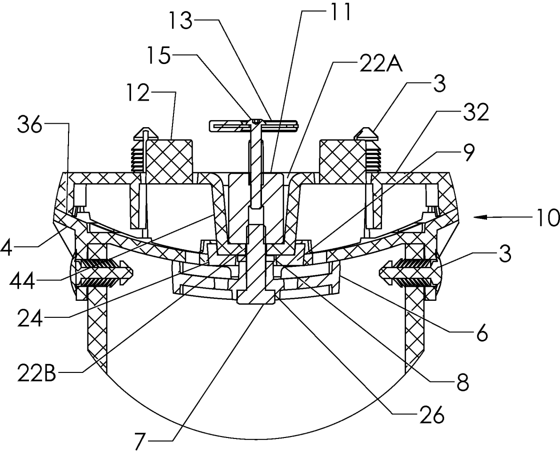
DETAIL C
