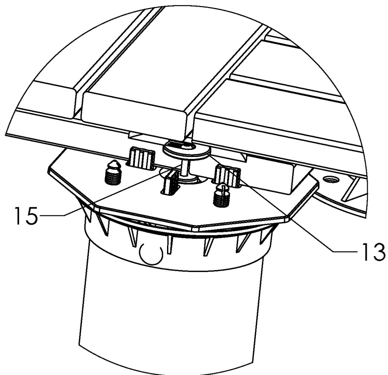
DETAIL B
