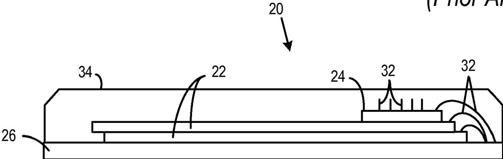
Fig. 1 (Prior Art)
