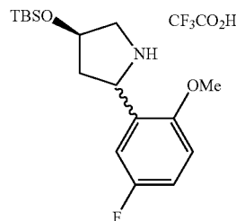
(R)-4-((tert-butyldimethylsilyl)oxy)-2-(5-fluoro-2-methoxyphenyl)pyrrolidine 2,2,2-trifluoroacetate
