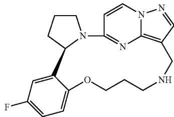
(6R)-9-fluoro-13-oxa-2,17,21,22,25-pentaazapentacyclo[17.5.2.0 2,6 .0 7,12 .0 22,26 ]]hexacos-1(25),7,9,11,19(26),20,23-heptaene
