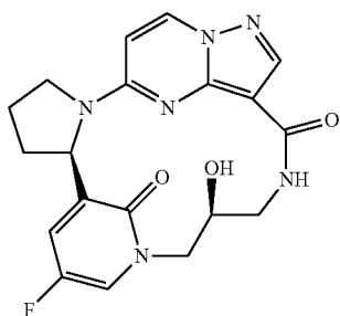
(6R,13S)-9-fluoro-13-hydroxy-2,11,15,19,20,23-hexaazapentacyclo-[15.5.2.1 7,11 .0 2,6 .0 20,24 ]pentacos-1(23),7,9,17(24),18,21-hexaene-16,25-dione
