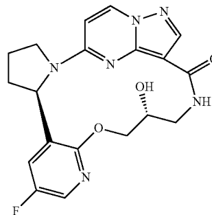
(6R,15R)-9-fluoro-15-hydroxy-13-oxa-2,11,17,21,22,25-hexaazapentacyclo-[17.5.2.0 2,6 .0 7,12 .0 22,26 ]hexacos-1(25),7,9,11,19(26),20,23-heptaen-18-one
