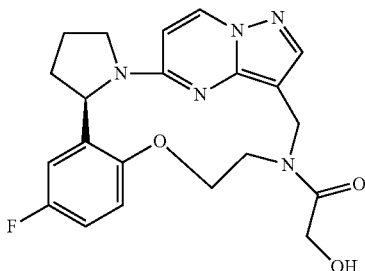
1-[(6R)-9-fluoro-13-oxa-2,16,20,21,24-pentaazapentacyclo[16.5.2.0 2,6 .0 7,12 .0 21,25 ]]pentacos-1(24),7,9,11,18(25),19,22-heptaen-16-yl]-2-hydroxyethan-1-one
