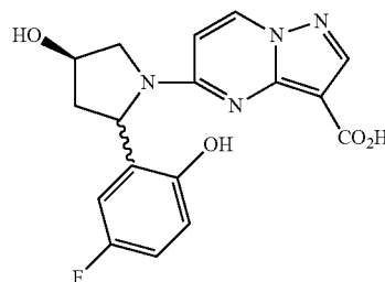
(R)-5-(2-(5-fluoro-2-hydroxyphenyl)-4-hydroxypyrrolidin-1-yl)pyrazolo[1,5-a]pyrimidine-3-carboxylic acid
