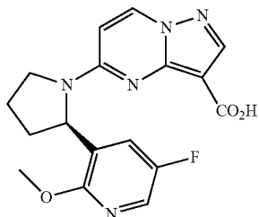
(R)-5-(2-(5-fluoro-2-methoxypyridin-3-yl)pyrrolidin-1-yl)pyrazolo[1,5-a]pyrimidine-3-carboxylic acid
