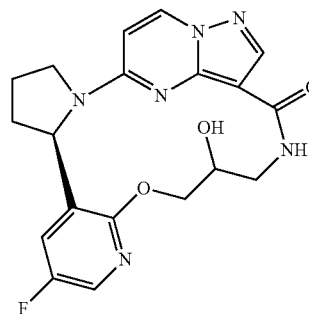
(6R)-9-fluoro-15-hydroxy-13-oxa-2,11,17,21,22,25-hexaazapentacyclo-[17.5.2.0 2,6 .0 7,12 .0 22,26 ]hexacos-1(25),7,9,11,19(26),20,23-heptaen-18-one
