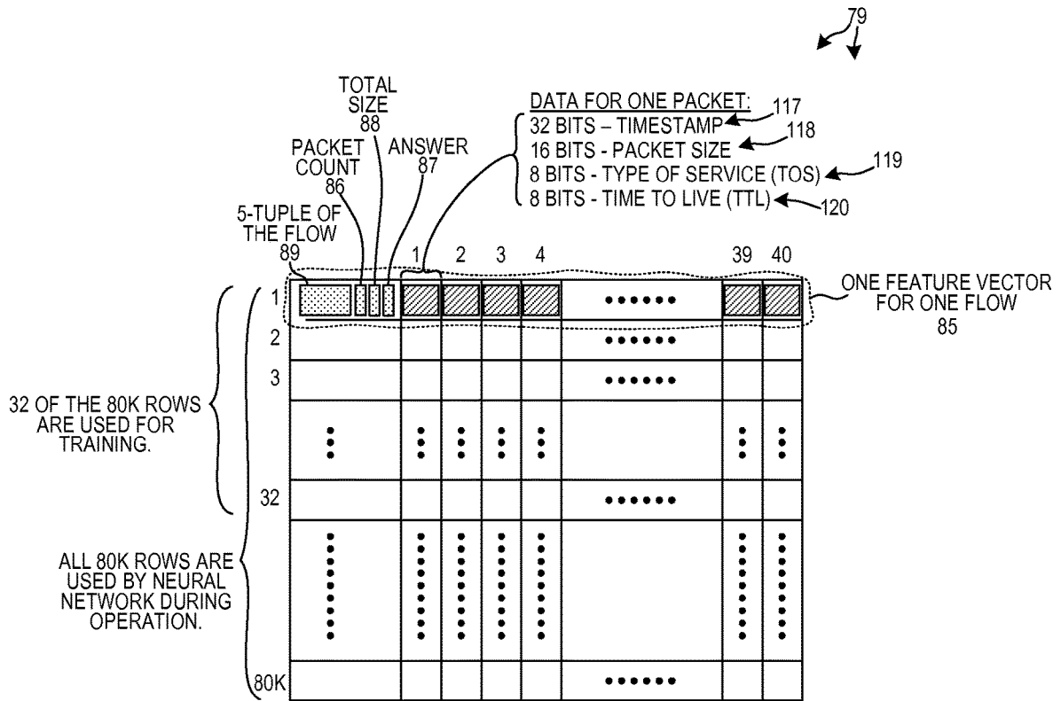
FEATURE VECTOR TABLE
