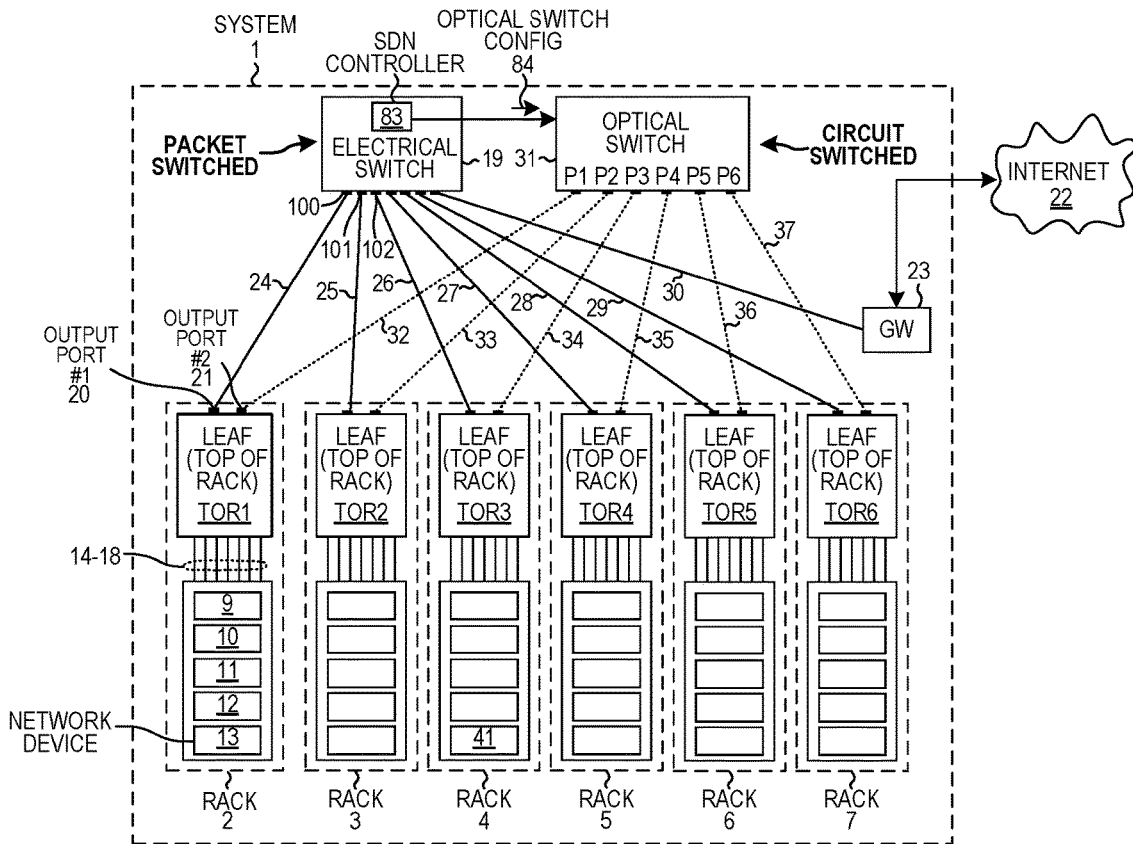
DATA CENTER
