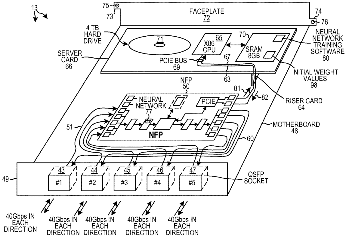
NETWORK DEVICE FIG. 6
