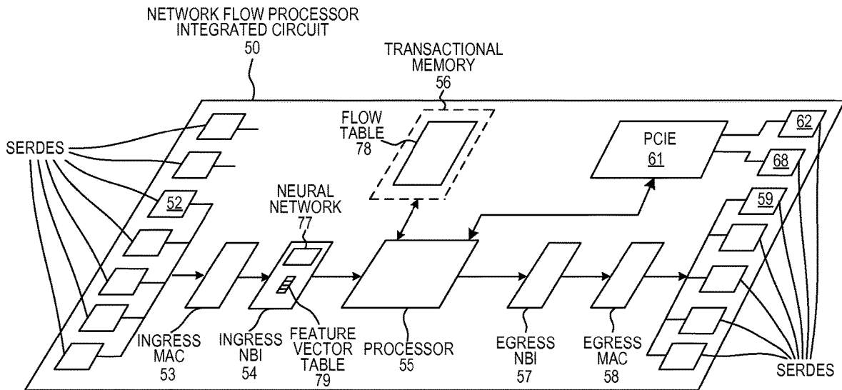
NETWORK FLOW PROCESSOR FIG. 7
