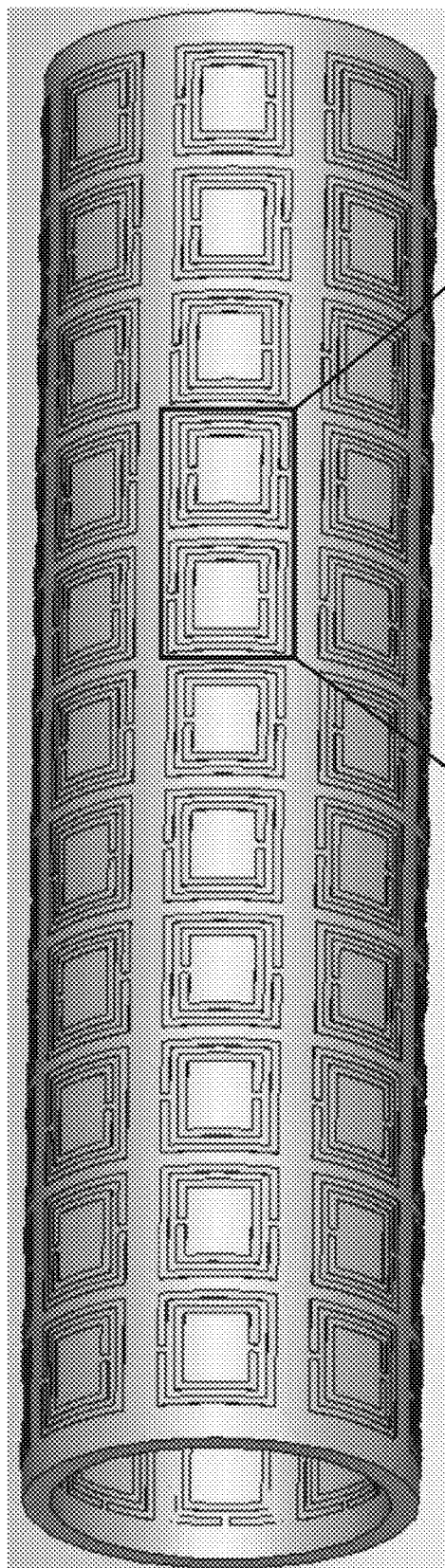
Cylindrical Metamaterial Polarizer 410
