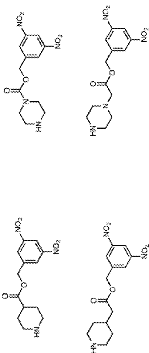
Cyclic secondary amines
