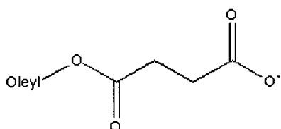
Compound I
