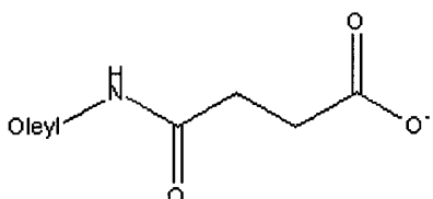
Compound V
