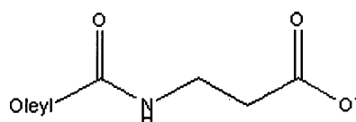
Compound IV
