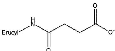
Compound III
