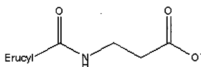
Compound II
