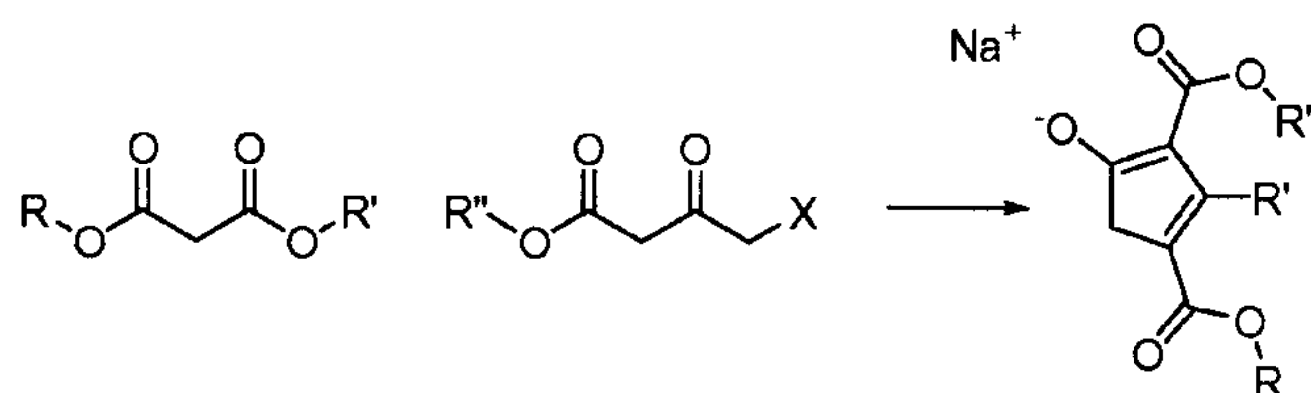
Scheme 29: Decarboxylation of a β-ketoester enolate (General Procedure CC)
