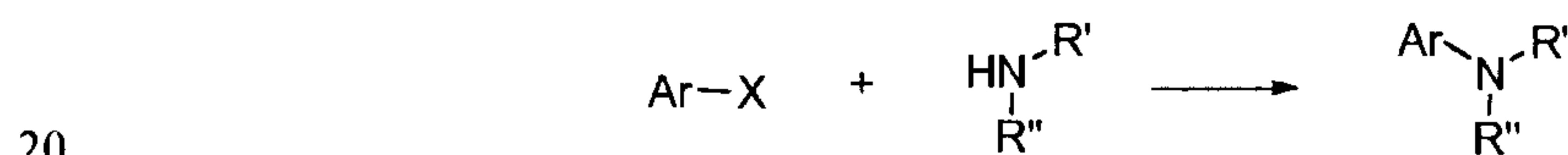
Scheme 15. Displacement of an aryl or heteroaryl halide with an amine (General Procedures O and O.1)
