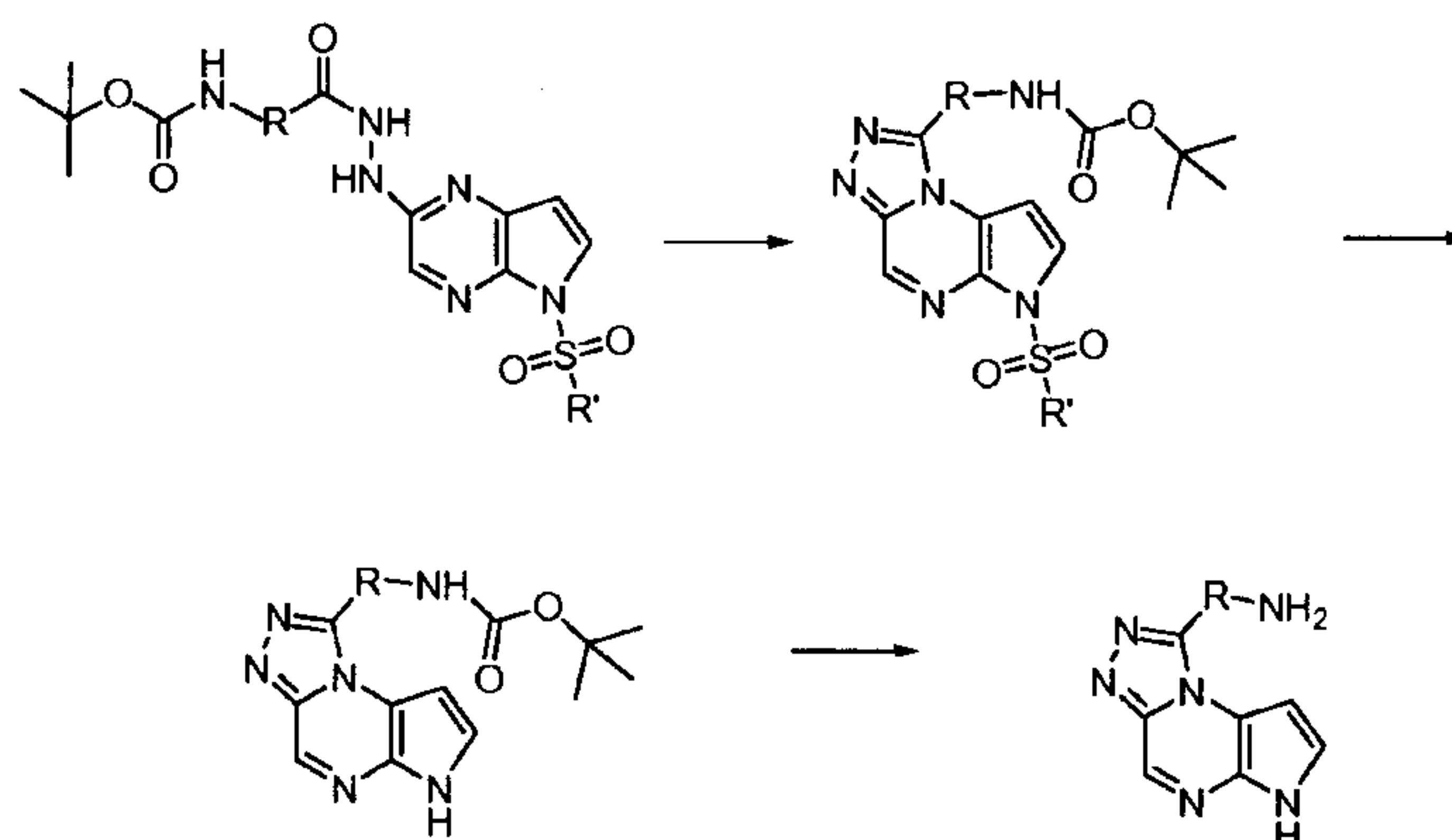
Scheme 5. Cyclization of a hydrazide followed by sulfonamide hydrolysis (General Procedure E)
