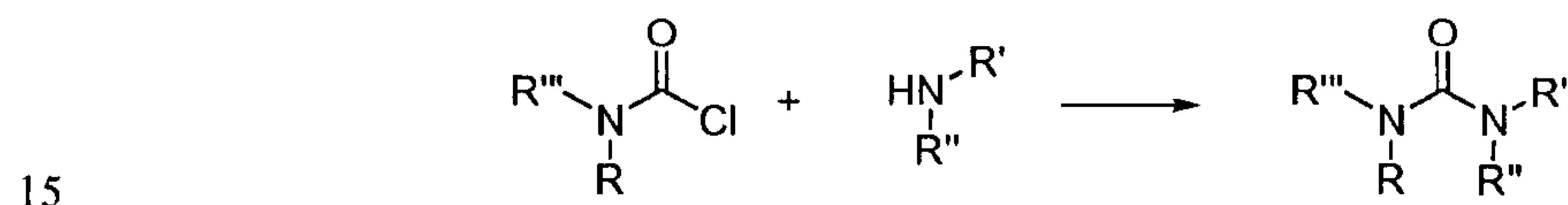
Scheme 14. Formation of a sulfonamide from an amine (General Procedure N)
