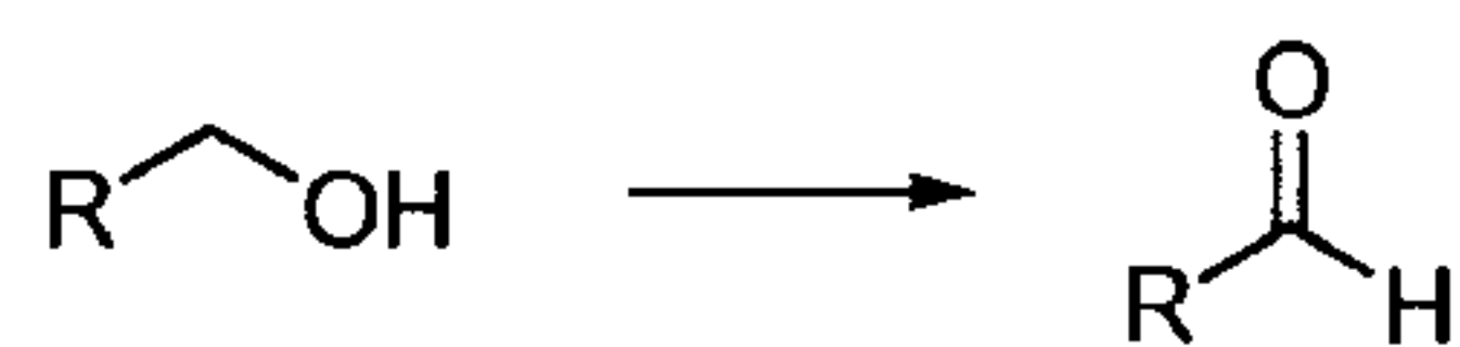
Scheme 21. Formation of a semicarbazide (General Procedure U)
