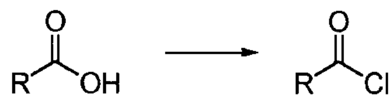
15 Scheme 23. Formation of an acid chloride (General Procedure W)
