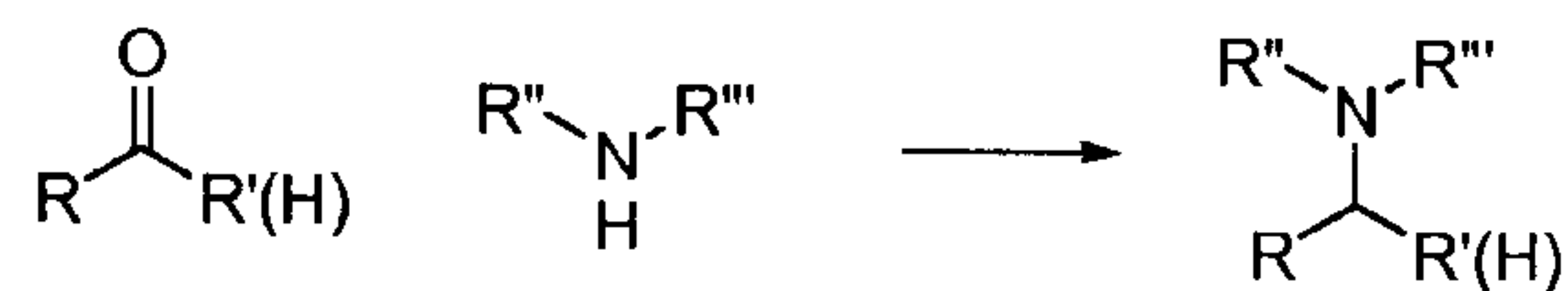
Scheme 32: Debenzylation of an amine (General Procedure FF)
