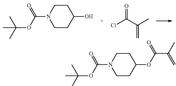
Scheme 1: Synthesis of TBPMA(N-t-BOC-piperidi-4-ol methacrylate)
