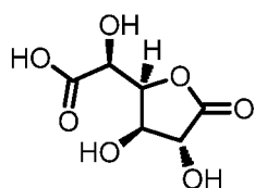
Glucaro-1,4-lactone
