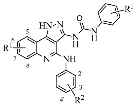
Formula II
