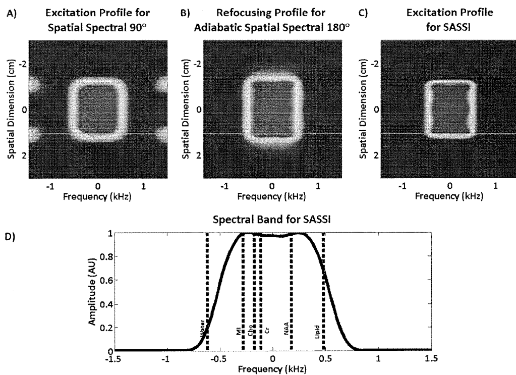
FIGS. 4A-4D
