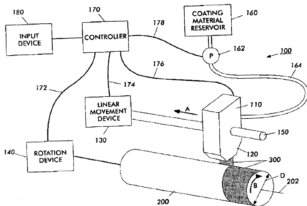
Figure 3: Schematic of a Rotary Cast Apparatus
