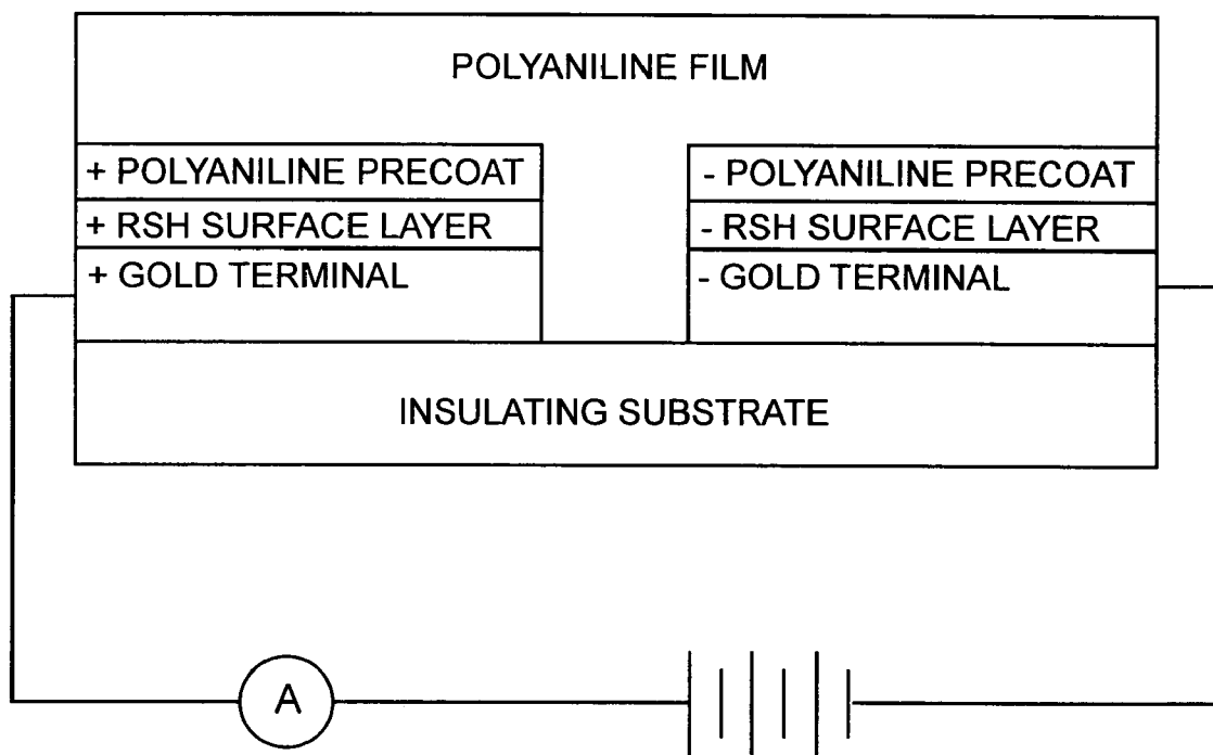
POLYANILINE NANOFIBER PRECOATED SENSOR
