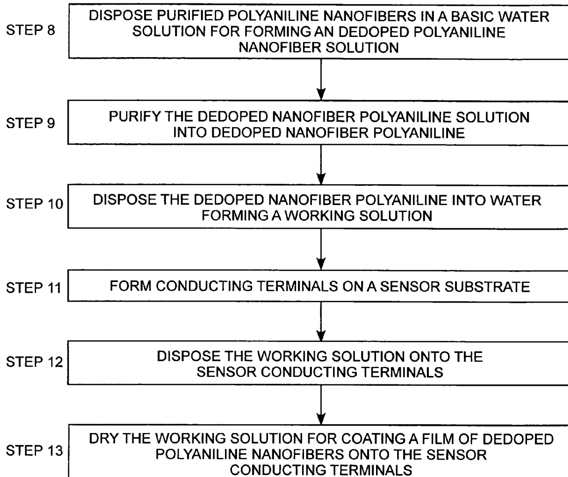
METHOD OF FORMING AN ACID SENSOR
