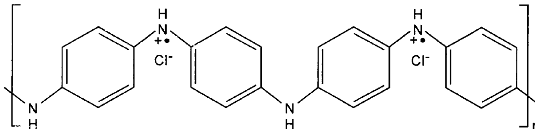
DOPED POLYANILINE EMERALDINE SALT ( \sigma = 10 \text{ S/cm} )
