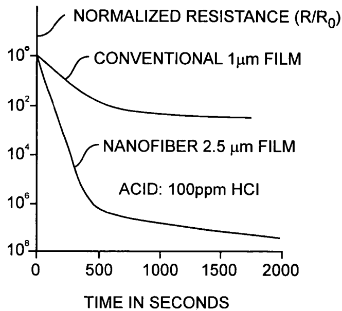
NANOFIBER TIME RESPONSE TO ACID DOPANT FIG. 4A
