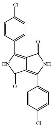
Pigment Red 254
