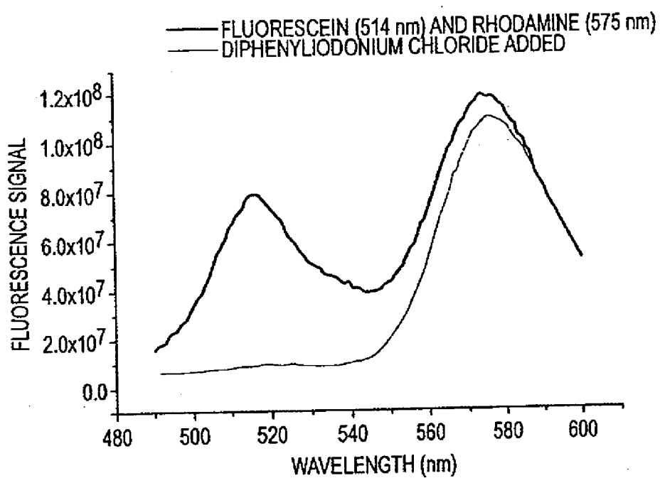
FLUORESCENCE SPECTRA OF EQUIMOLAR FLUORESCCEIN AND TETRAMETHYLRHODAMINE BEFORE AND AFTER ADDITION OF DIPHENYLIODONIUM CHLORIDE
