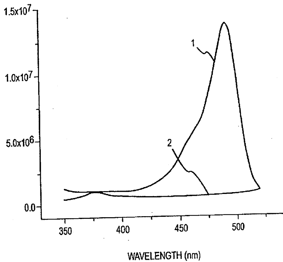
UV ABSORPTION SPECTRA: (1) FLUORESCIN (2) FLUORESCIN + DPI AFTER SINGLE FLASH FROM CAMERA STROBE
