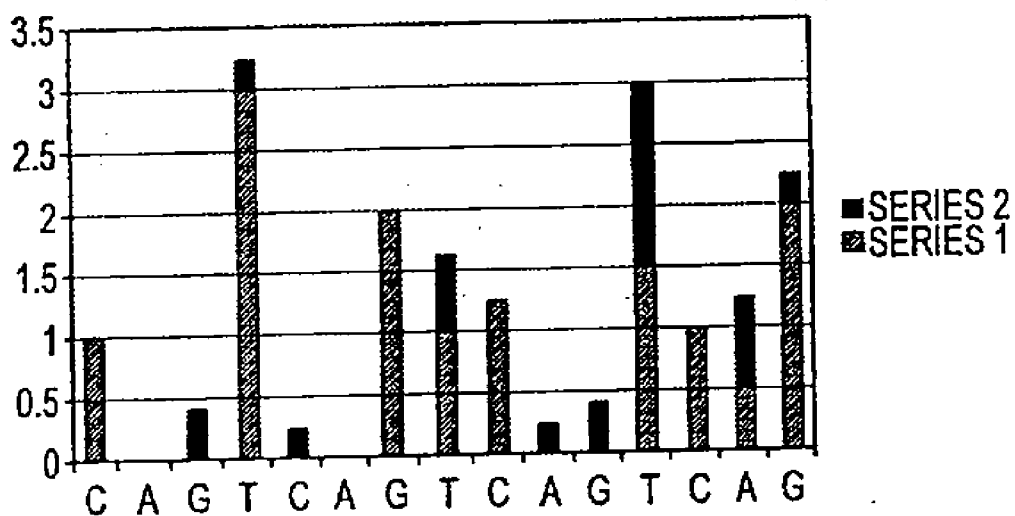
EFFECT OF A LEADING STRAND POPULATION ON EXTENSION SIGNALS
