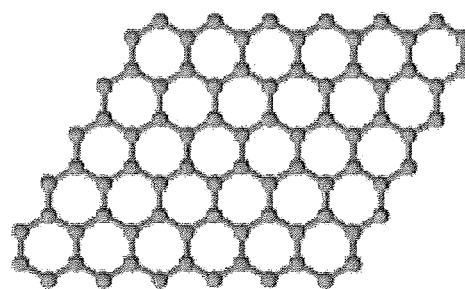
Graphene
