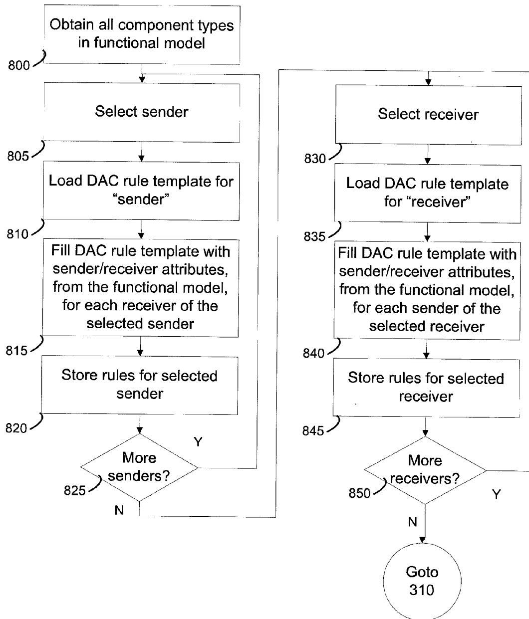
Fig. 8 DAC-Rule Generation Example
