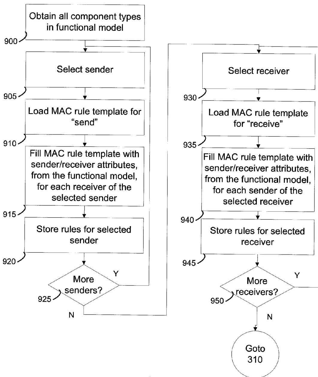
Fig. 9 MAC-Rule Generation Example
