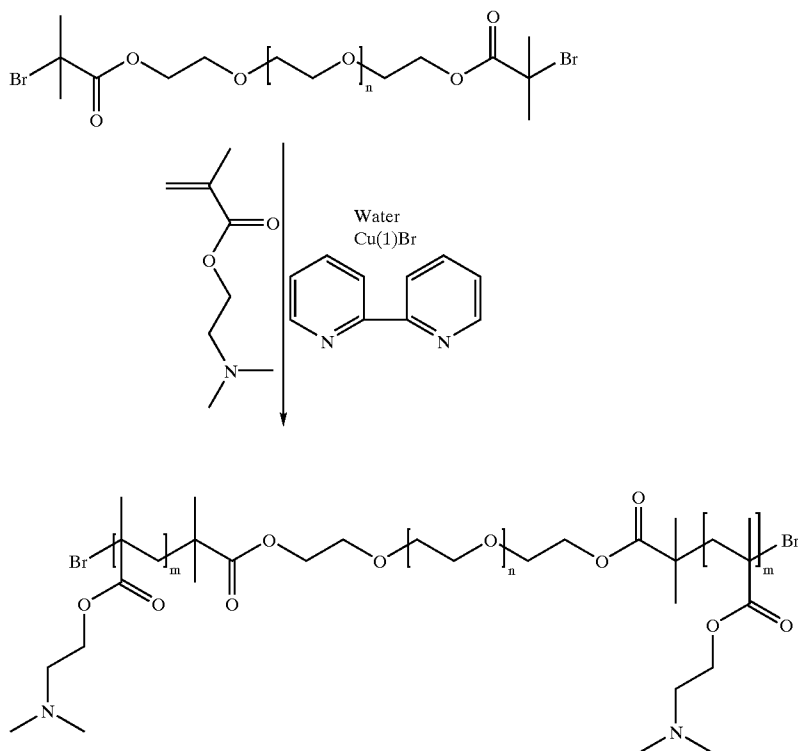
Reaction scheme 2:
