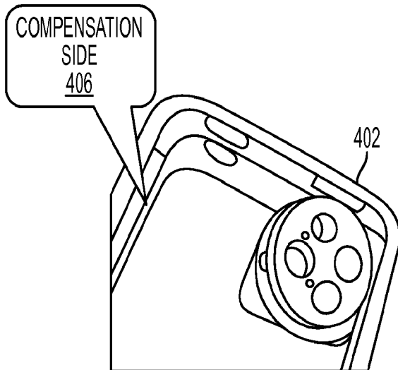
INSERTION OF CAROUSEL TO CASE
