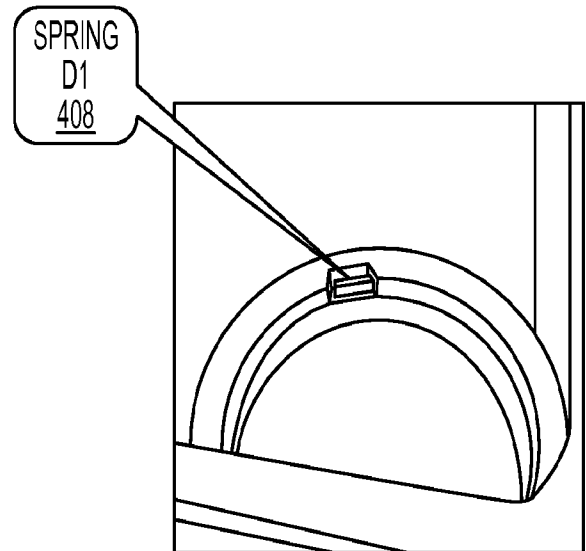
CAROUSEL LOCATION HOLE WITH ANNULAR SLIDER SURFACE AND CAROUSEL LOCATOR AND LOCK SPRING
