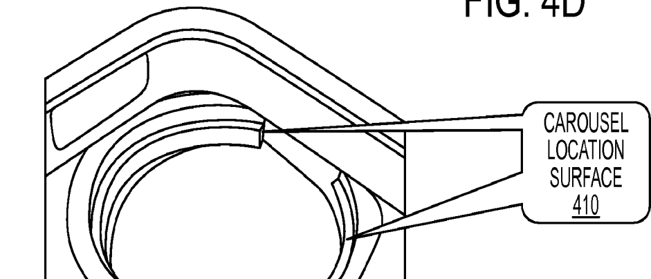
CAROUSEL HOLE WITH SEMI-ANNULAR SLIDER SURFACE AND CASE EDGE MARGIN THAT COOPERATES TO FIX THE CAROUSEL POSITION
