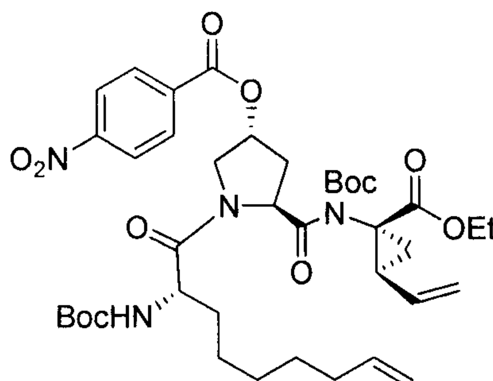
(3R,5S)-5-(tert-butoxycarbonyl((1R)-1-(ethoxycarbonyl)-2-vinylcyclopropyl)carbamoyl)-1-((S)-2-(tert-butoxycarbonylamino)non-8-enoyl)pyrrolidin-3-yl 4-nitrobenzoate
