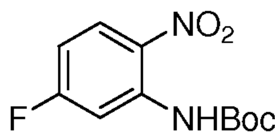
tert -butyl 5-fluoro-2-nitrophenylcarbamate
