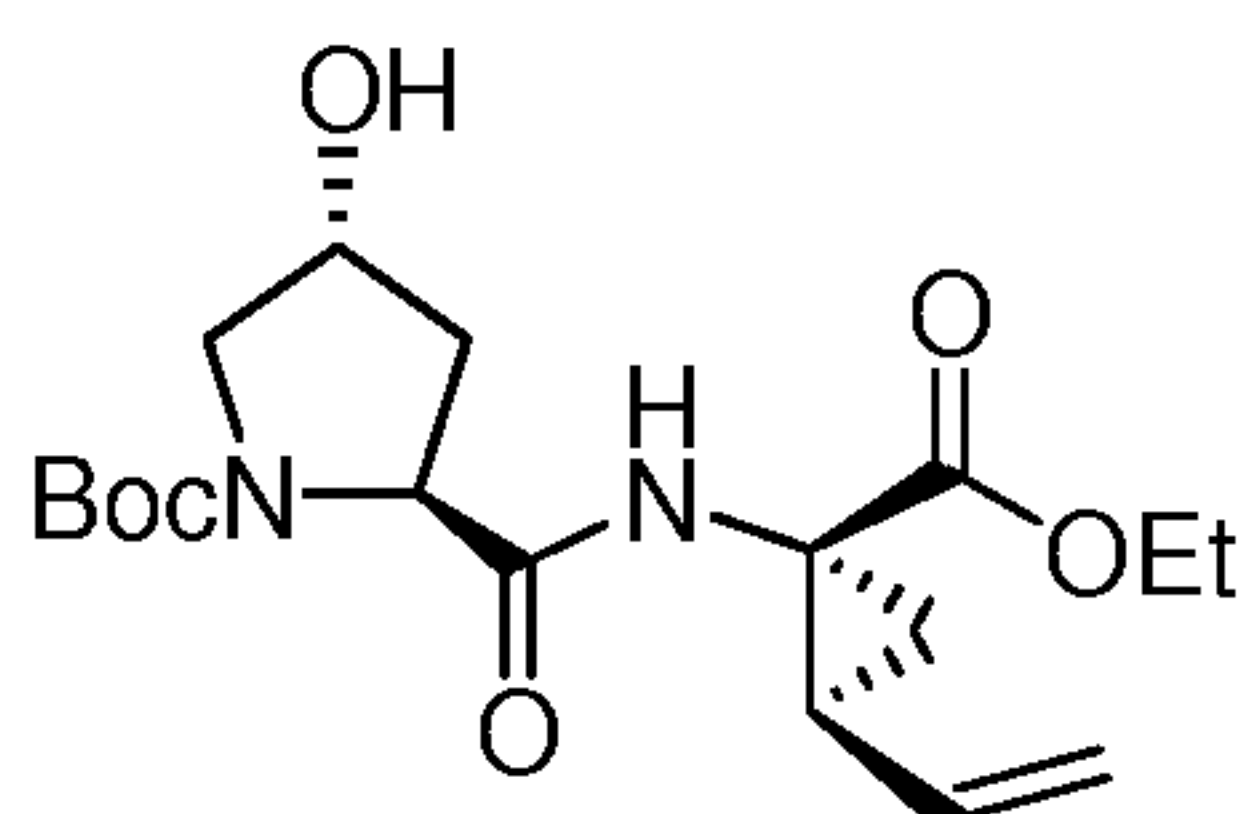
(2S,4R)-tert-butyl 2-(((1R,2S)-1-(ethoxycarbonyl)-2-vinylcyclopropyl)carbamoyl)-4- hydroxypyrrolidine-1-carboxylate
