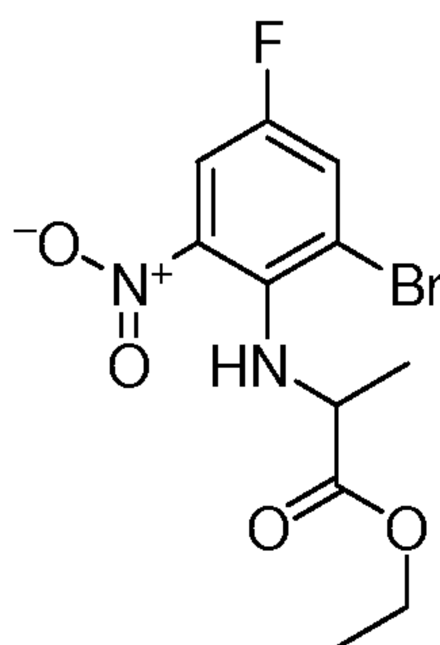
ethyl 2-(2-bromo-4-fluoro-6-nitrophenylamino)propanoate
