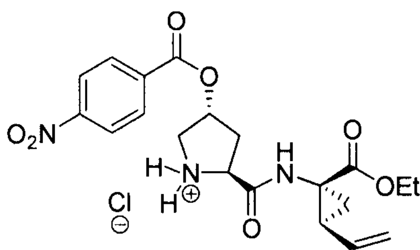
(2S,4R)-2-((1R,2S)-1-(ethoxycarbonyl)-2-vinylcyclopropylcarbamoyl)-4-(4-nitrobenzoyloxy)pyrrolidinium chloride
