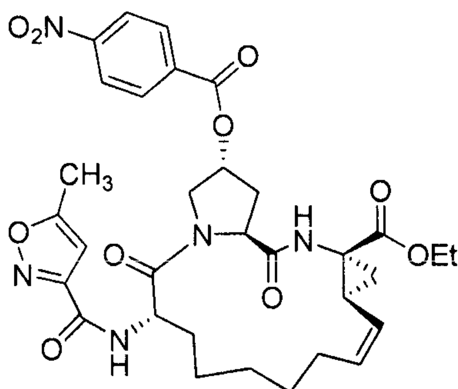
(2R,6S,13aS,14aR,16aS,Z)-ethyl 6-(5-methylisoxazole-3-carboxamido)-2-(4-nitrobenzoyloxy)-5,16-dioxo-1,2,3,5,6,7,8,9,10,11,13a,14,14a,15,16,16a-hexadecahydrocyclopropa[e]pyrrolo[1,2-a][1,4]diazacyclopentadecine-14a-carboxylate
