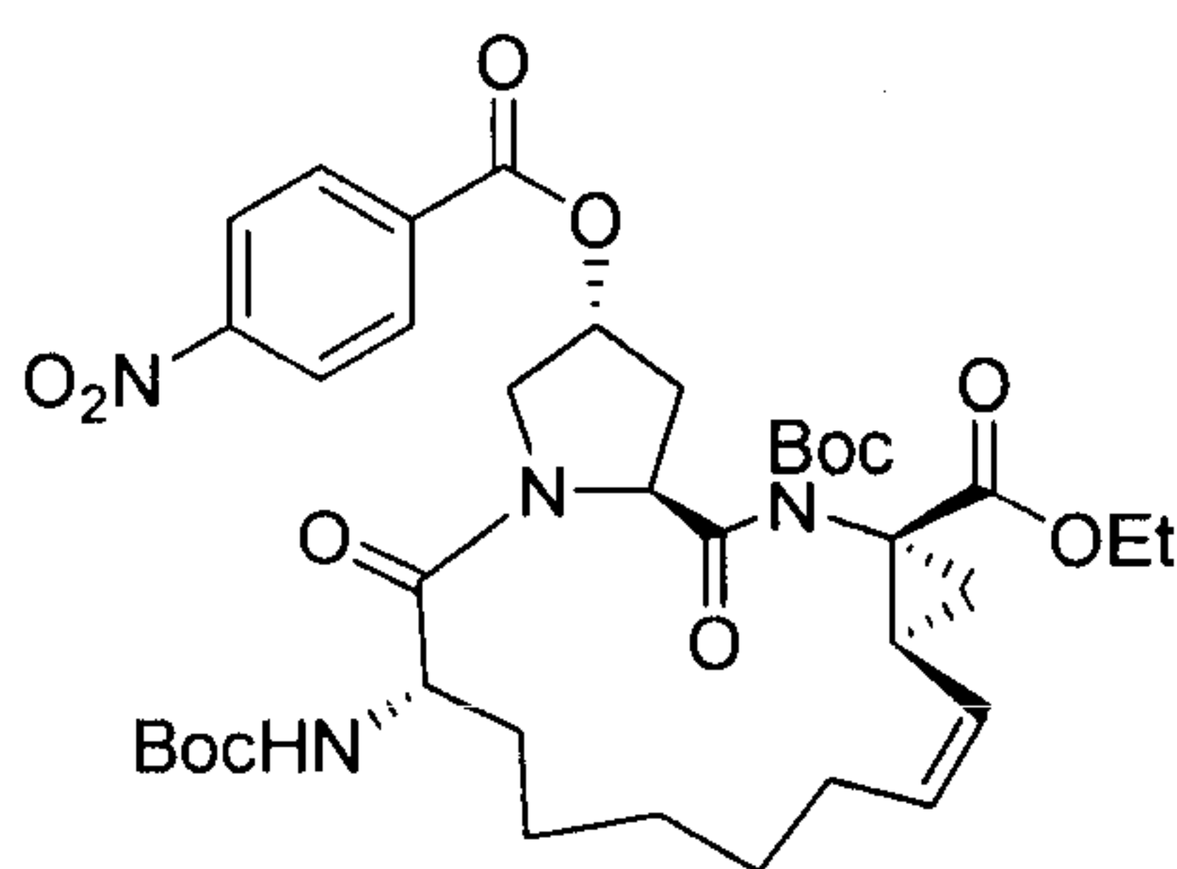
(2R,6S,14aR,16aS,Z)-15-tert-butyl 14a-ethyl 6-(tert-butoxycarbonylamino)-2-(4-nitrobenzoyloxy)-5,16-dioxo-2,3,5,6,7,8,9,10,11,13a,14,14a,16,16a-tetradecahydrocyclopropa[e]pyrrolo[1,2-a][1,4]diazacyclopentadecine-14a,15(1H)-dicarboxylate
