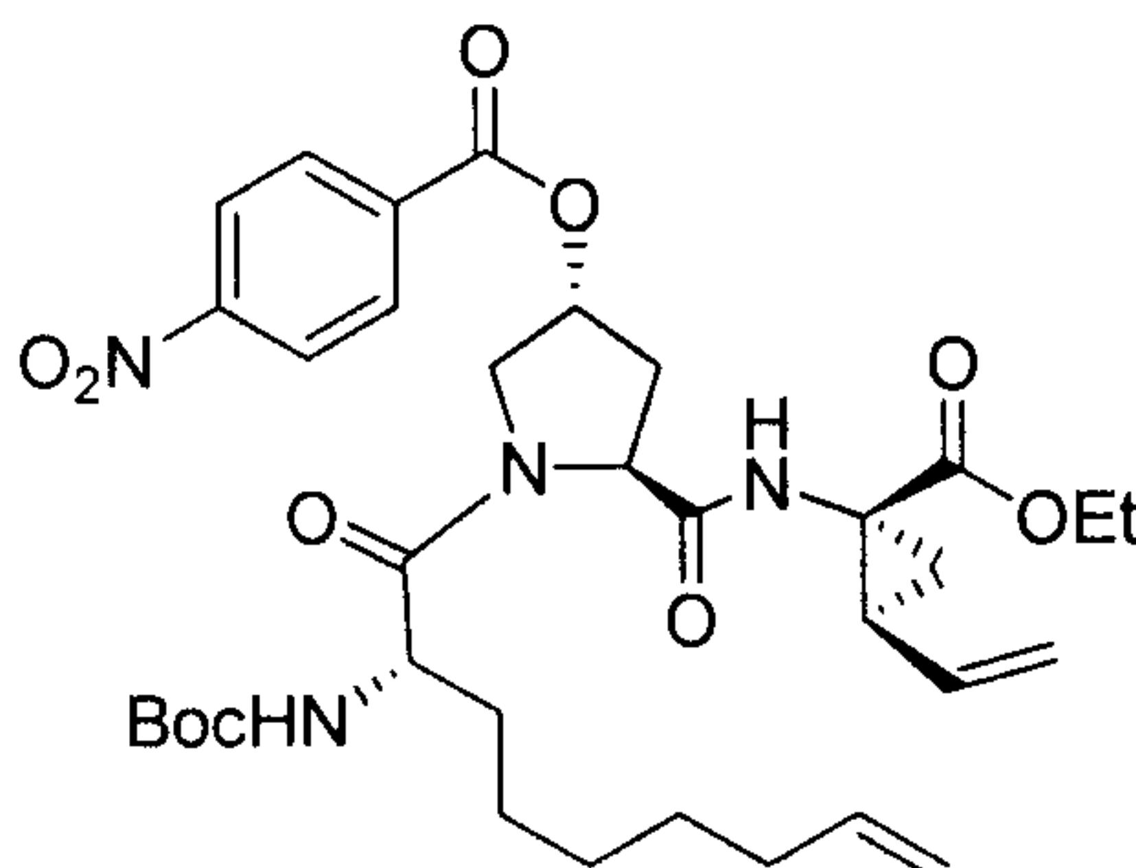
(3R,5S)-1-((S)-2-(tert-butoxycarbonylamino)non-8-enoyl)-5-((1R,2S)-1-(ethoxycarbonyl)-2-vinylcyclopropylcarbamoyl)pyrrolidin-3-yl 4-nitrobenzoate
