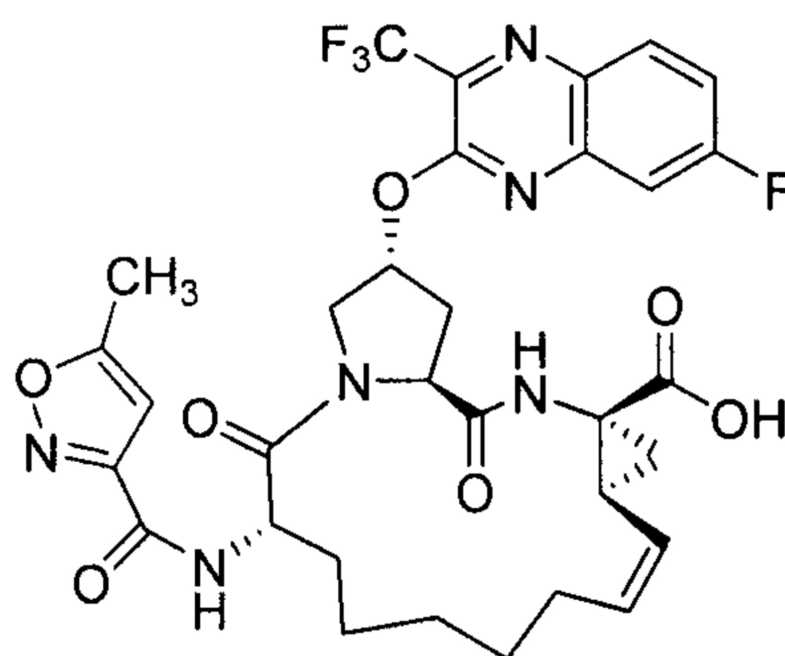
(2R,6S,13aS,14aR,16aS,Z)-2-(7-fluoro-3-(trifluoromethyl)quinoxalin-2-yloxy)-6-(5-methylisoxazole-3-carboxamido)-5,16-dioxo-1,2,3,5,6,7,8,9,10,11,13a,14,14a,15,16,16a-hexadecahydrocyclopropa[e]pyrrolo[1,2-a][1,4]diazacyclopentadecine-14a-carboxylic acid
