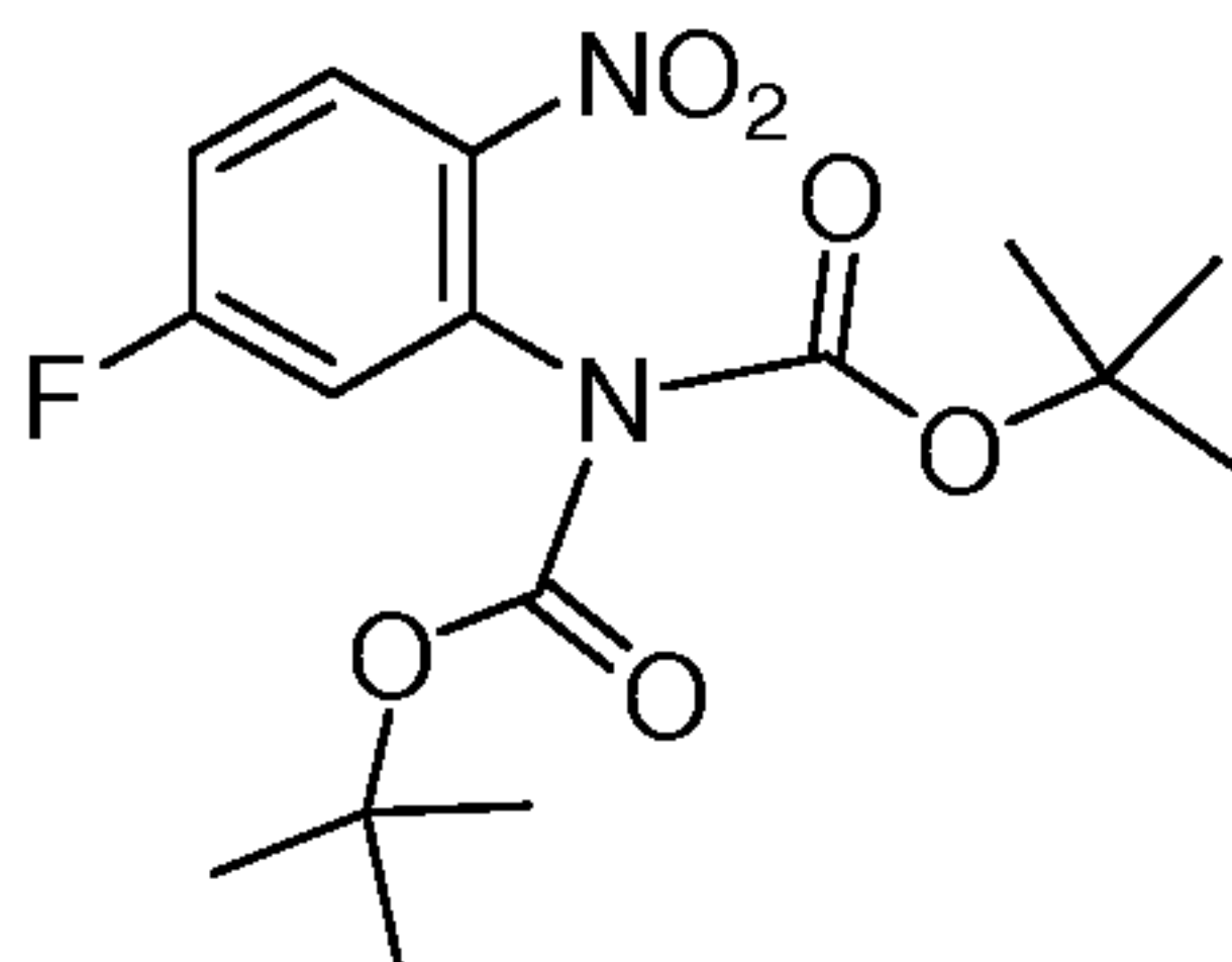
di- tert -butyl 5-fluoro-2-nitrophenyl dicarbamate
