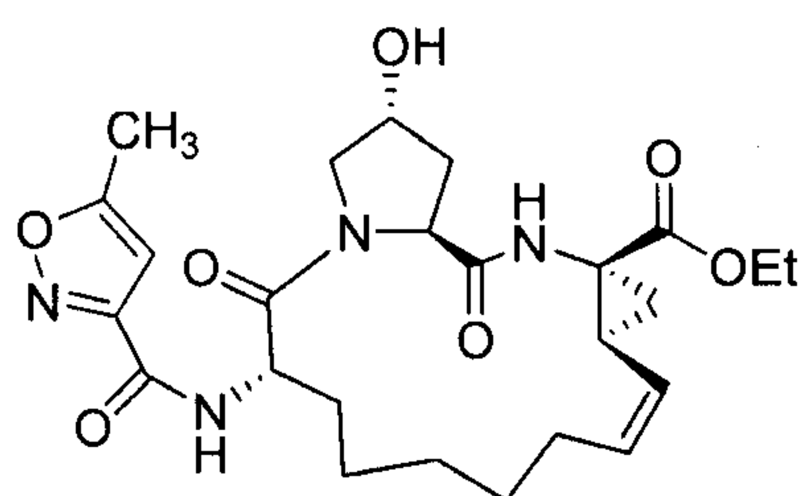
(2R,6S,14aR,16aS,Z)-ethyl 2-hydroxy-6-(5-methylisoxazole-3-carboxamido)-5,16-dioxo-1,2,3,5,6,7,8,9,10,11,13a,14,14a,15,16,16a-hexadecahydrocyclopropa[e]pyrrolo[1,2-a][1,4]diazacyclopentadecine-14a-carboxylate
