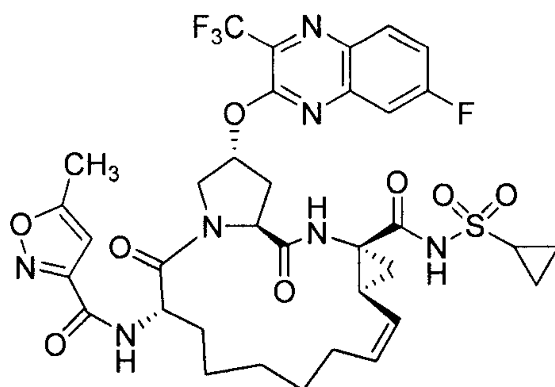
N-((2R,6S,13aS,14aR,16aS,Z)-14a-(cyclopropylsulfonylcarbamoyl)-2-(7-fluoro-3-(trifluoromethyl)quinoxalin-2-yloxy)-5,16-dioxo-1,2,3,5,6,7,8,9,10,11,13a,14,14a,15,16,16a-hexadecahydrocyclopropa[e]pyrrolo[1,2-a][1,4]diazacyclopentadecin-6-yl)-5-methylisoxazole-3-carboxamide
