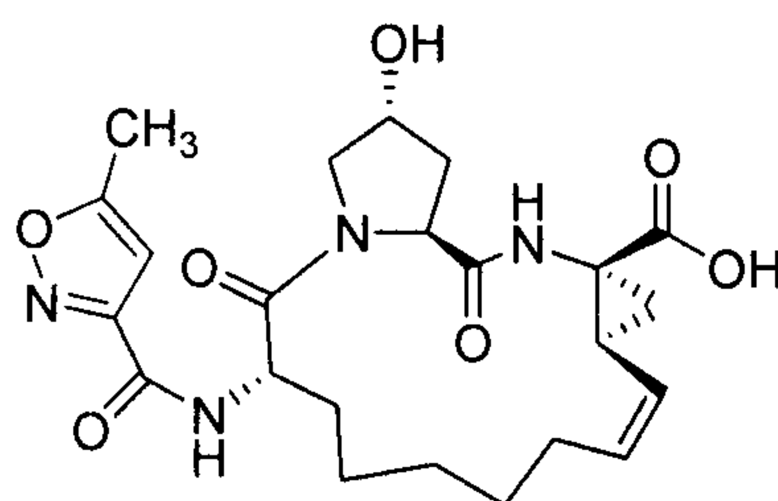
(2R,6S,14aR,16aS,Z)-2-hydroxy-6-(5-methylisoxazole-3-carboxamido)-5,16-dioxo-1,2,3,5,6,7,8,9,10,11,13a,14,14a,15,16,16a-hexadecahydrocyclopropa[e]pyrrolo[1,2-a][1,4]diazacyclopentadecine-14a-carboxylic acid
