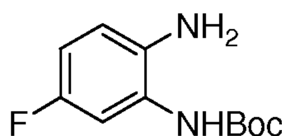
tert -butyl 2-amino-5-fluorophenylcarbamate
