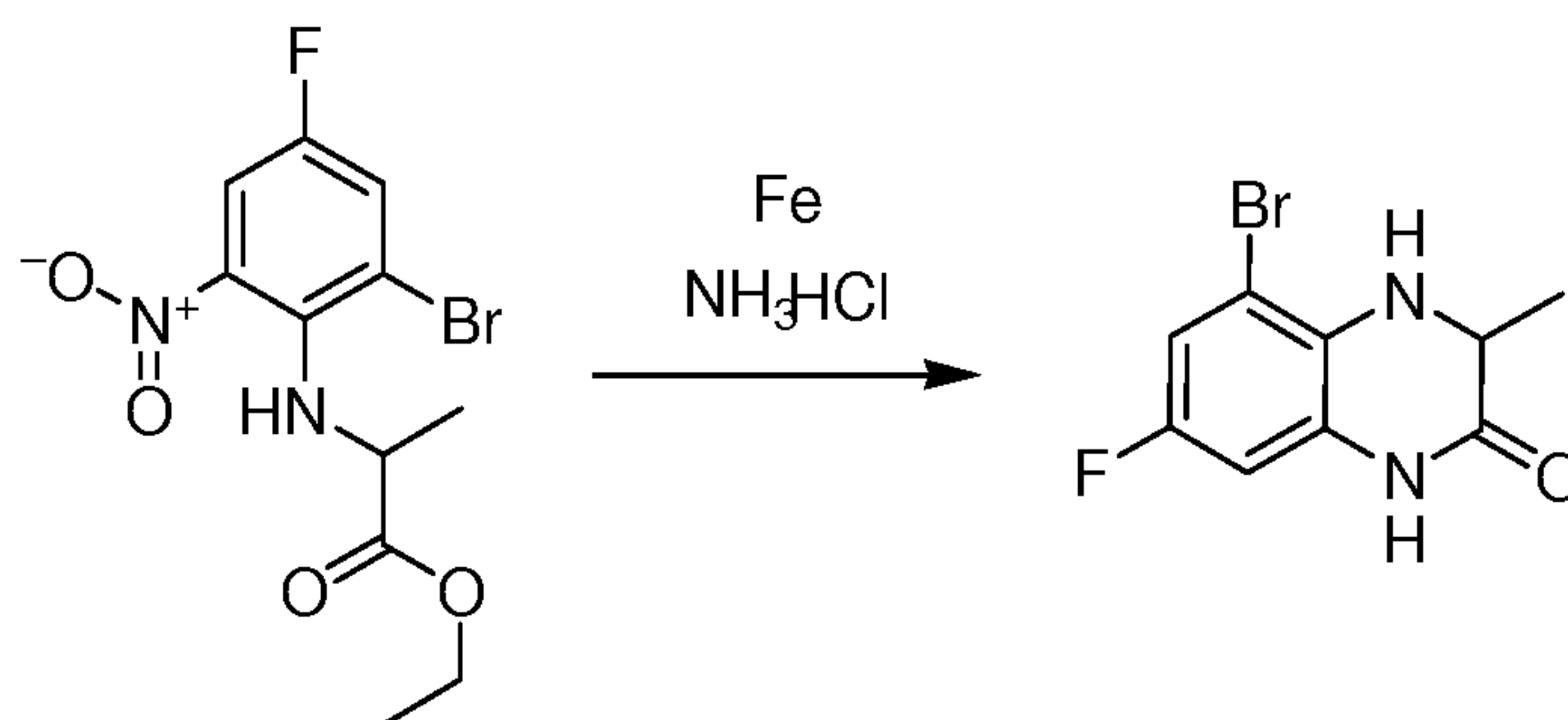
5-bromo-7-fluoro-3-methyl-3,4-dihydroquinoxalin-2(1H)-one
