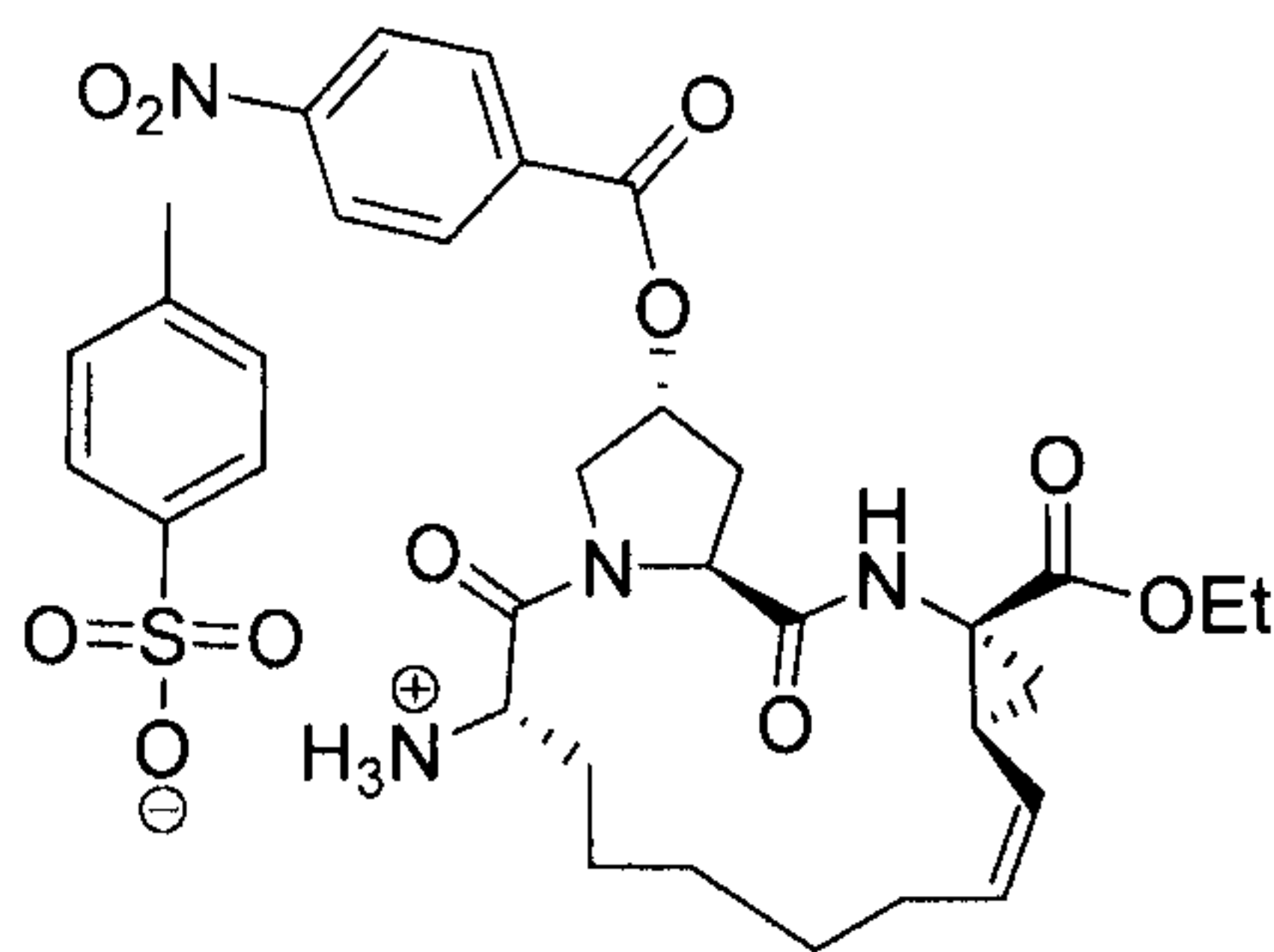
(2R,6S,13aS,14aR,16aS,Z)-14a-(ethoxycarbonyl)-2-(4-nitrobenzoyloxy)-5,16-dioxo-1,2,3,5,6,7,8,9,10,11,13a,14,14a,15,16,16a-hexadecahydrocyclopropa[e]pyrrolo[1,2-a][1,4]diazacyclopentadecin-6-aminium 4-methylbenzenesulfonate
