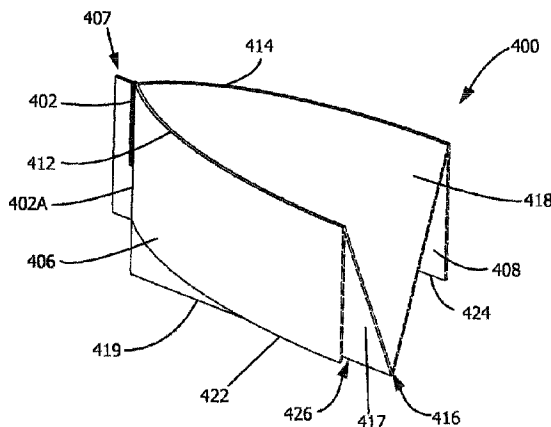
GUSSET TOP SIDE SEAL COVER WITH SHORT SIDES ( SECTION VIEW )
