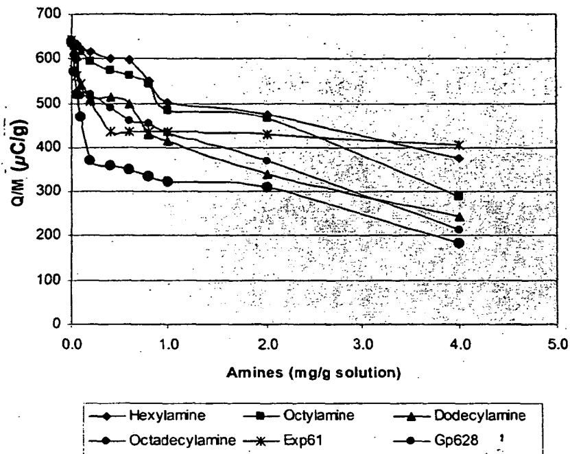
Figure 7, Effect of carbon chain length of the amines on Q/M value of a black toner particles.
