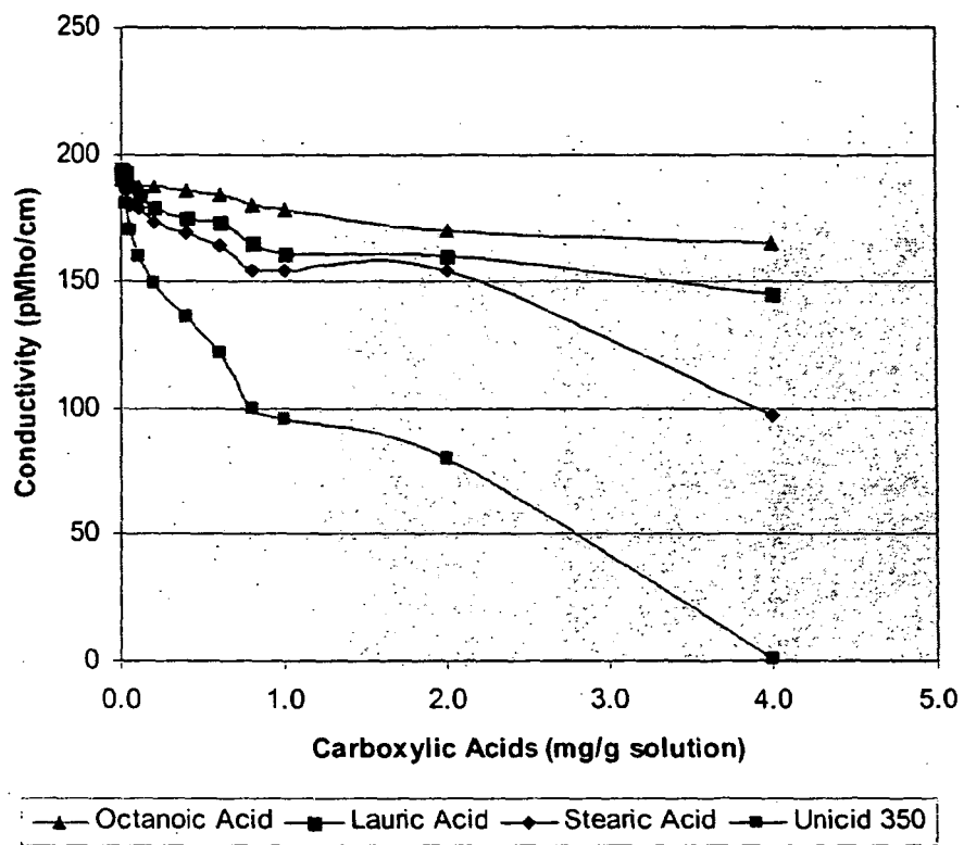
Figure 4, Effect of carbon chain length of carboxylic acids on bulk conductivity of the black toner.
