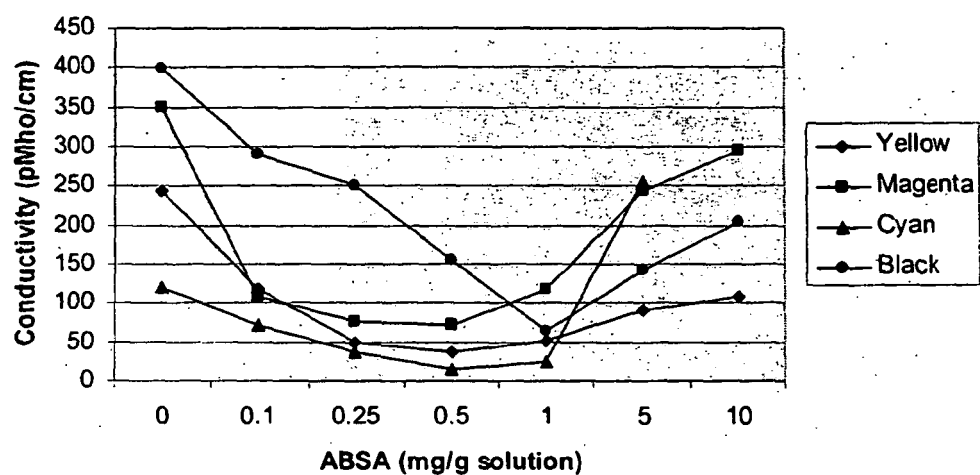
Figure 2, Toner bulk conductivity reduced with the amount of the addition of alkylbenzenesulfonic acid (ABSA, mixture of C 11 , C 12 and C 13 carbon chain length) in the depleted toner
