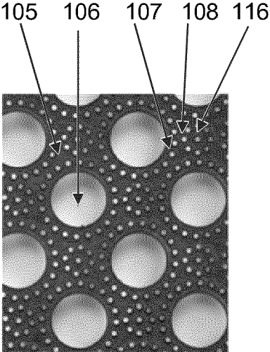
8 mm/1 mm voids, 60.7% ECA, 42.9% CA, 538 CFM
