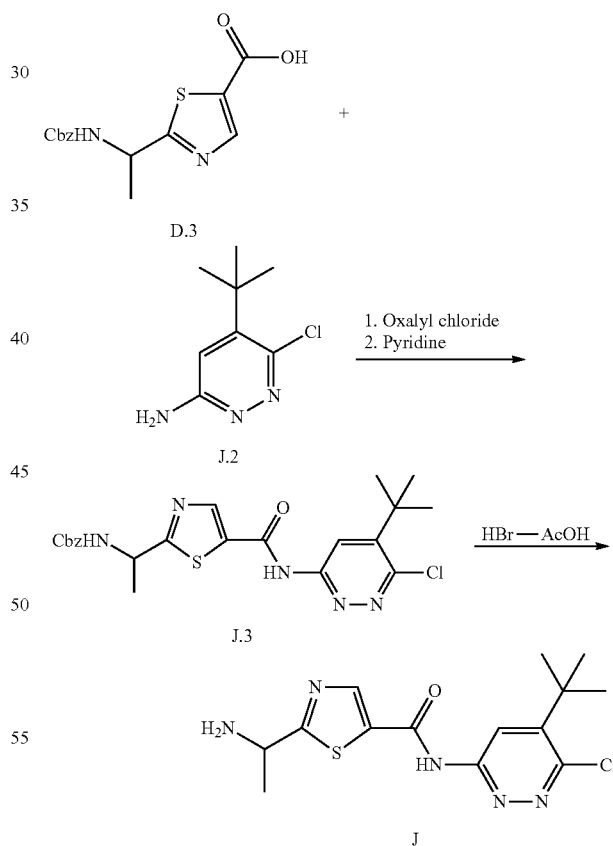
Scheme J-2.
