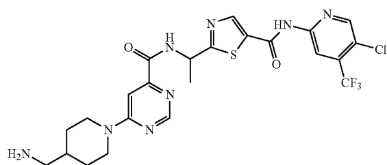
19ooD
