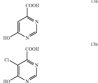
Scheme 13.
