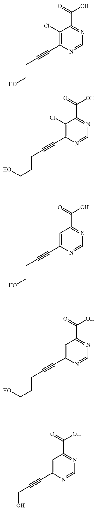
Scheme 8
