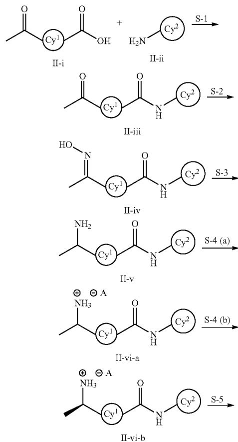
Scheme II
