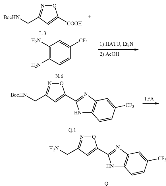
Scheme Q.
