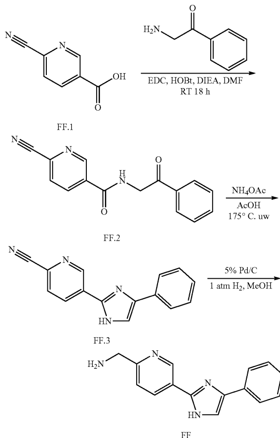
Scheme FF.
