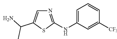
Scheme W.
