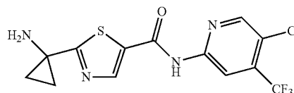
Scheme T
