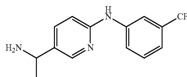
Scheme II.
