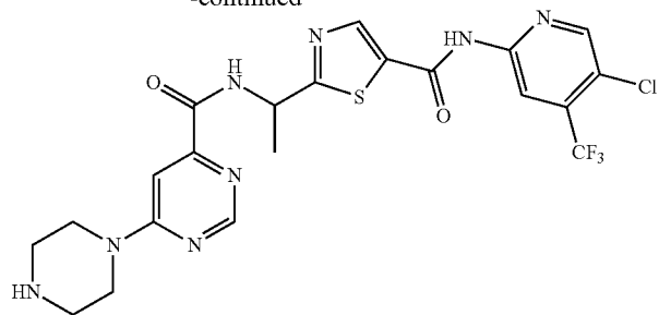
19iID
