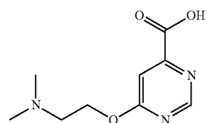
Scheme 19.1
