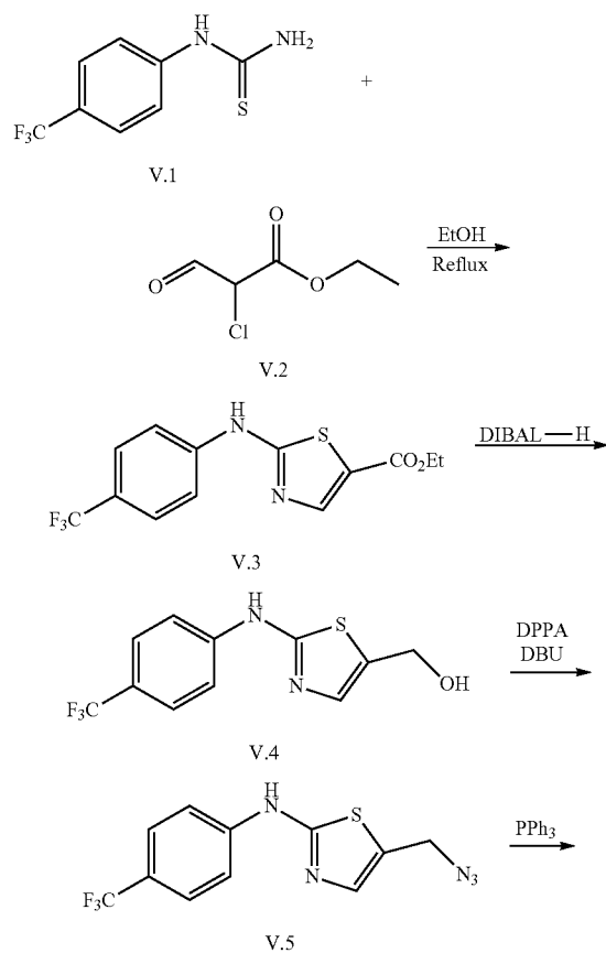
Scheme V.
