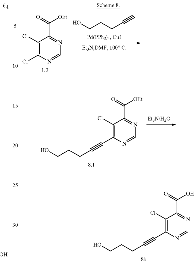
Scheme 8.
