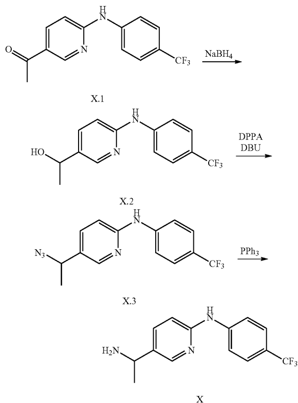
Scheme X.
