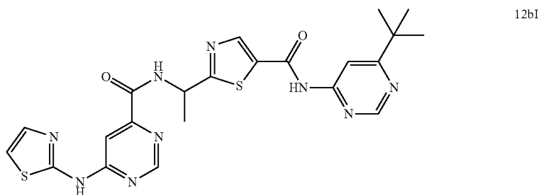
Exemplary Compounds of Formula I Additional compounds
