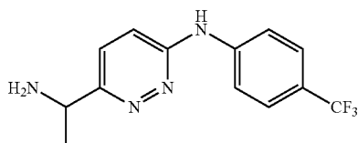
Scheme BB.
