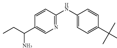
EE
