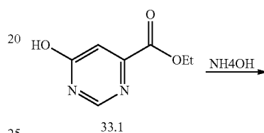
Scheme 33.
