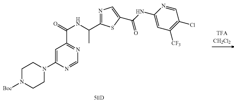
Scheme 19.1
