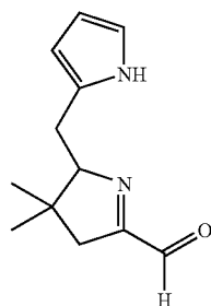
a tetrahydrodipyrin
