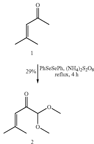
Scheme 2
