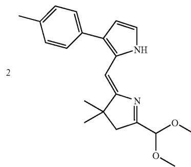
Scheme 6
