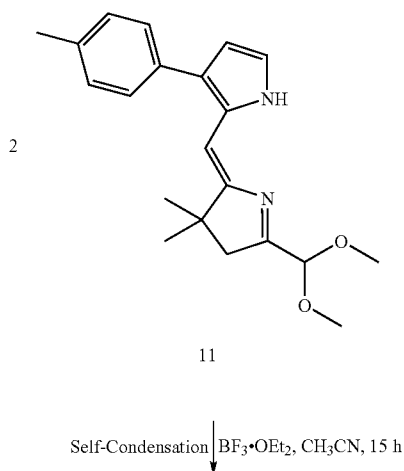
Scheme 4
