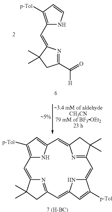
Scheme 9
