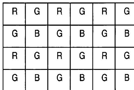
Bayer mosaic of several 2x2 pixel blocks
