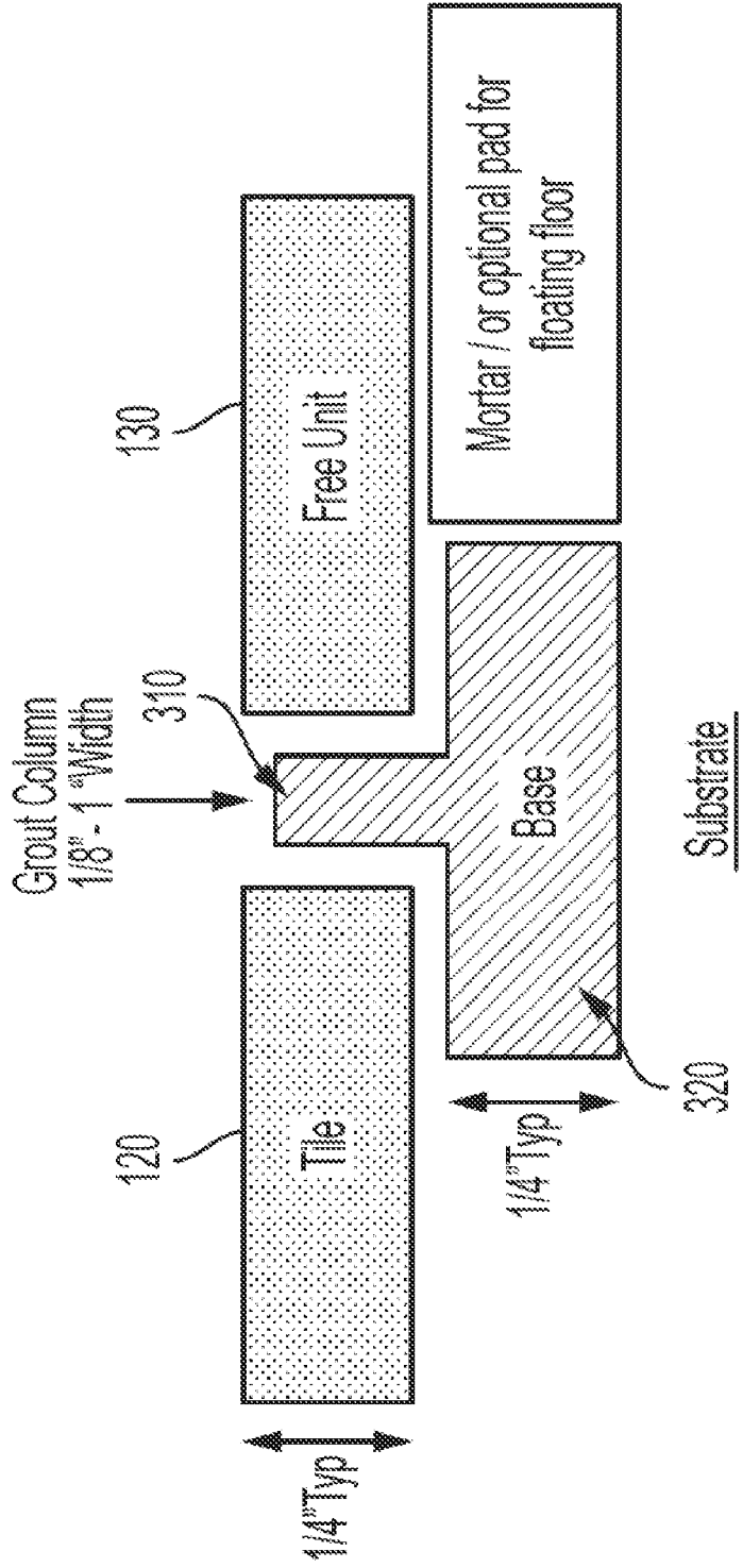
T-Bar Profile with tile
