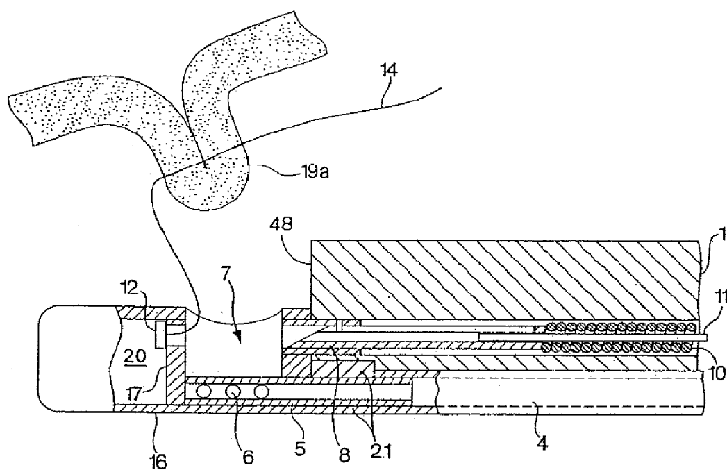
Fig. 3 (PRIOR ART)
