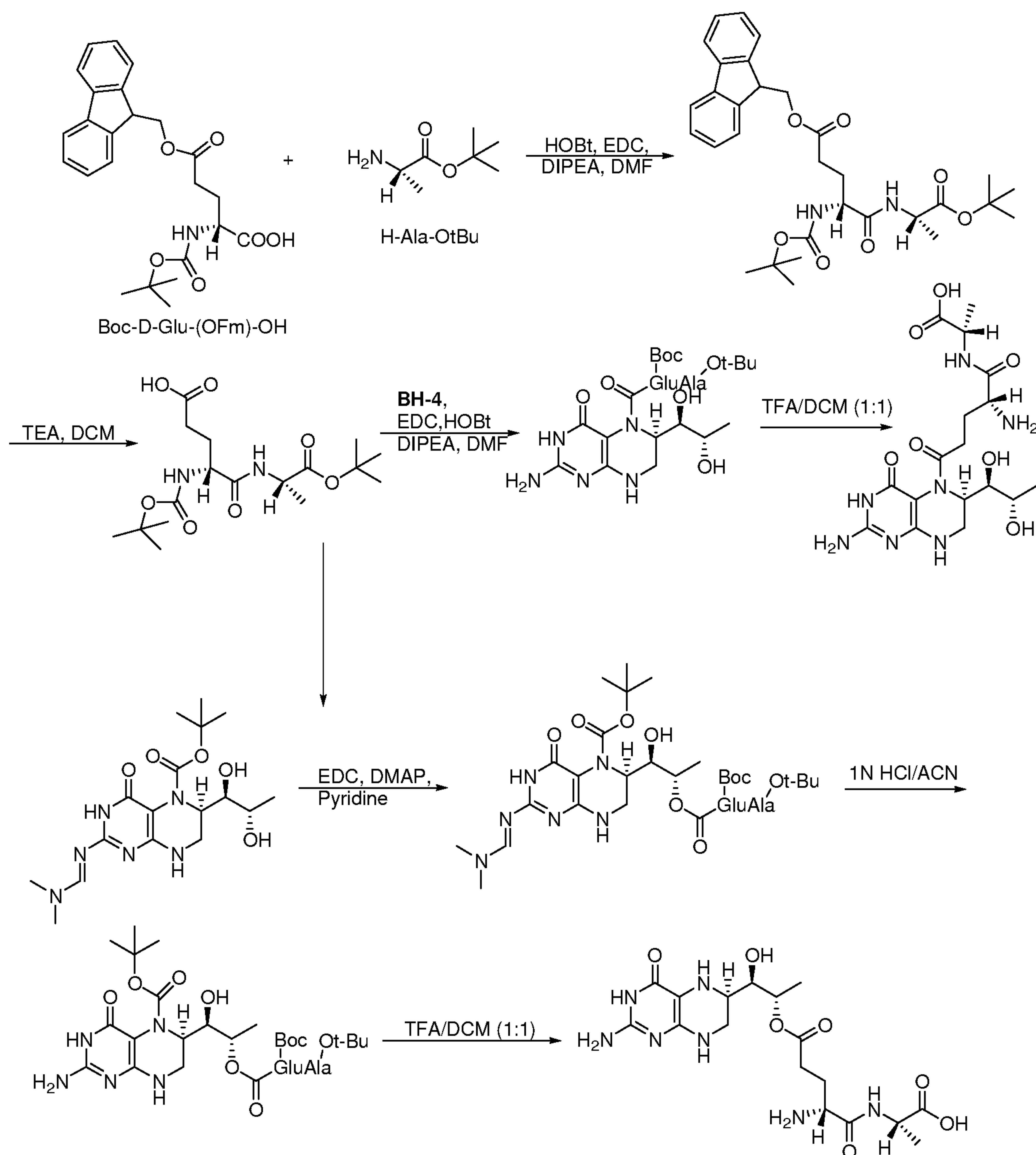
Reaction Scheme (IB)
