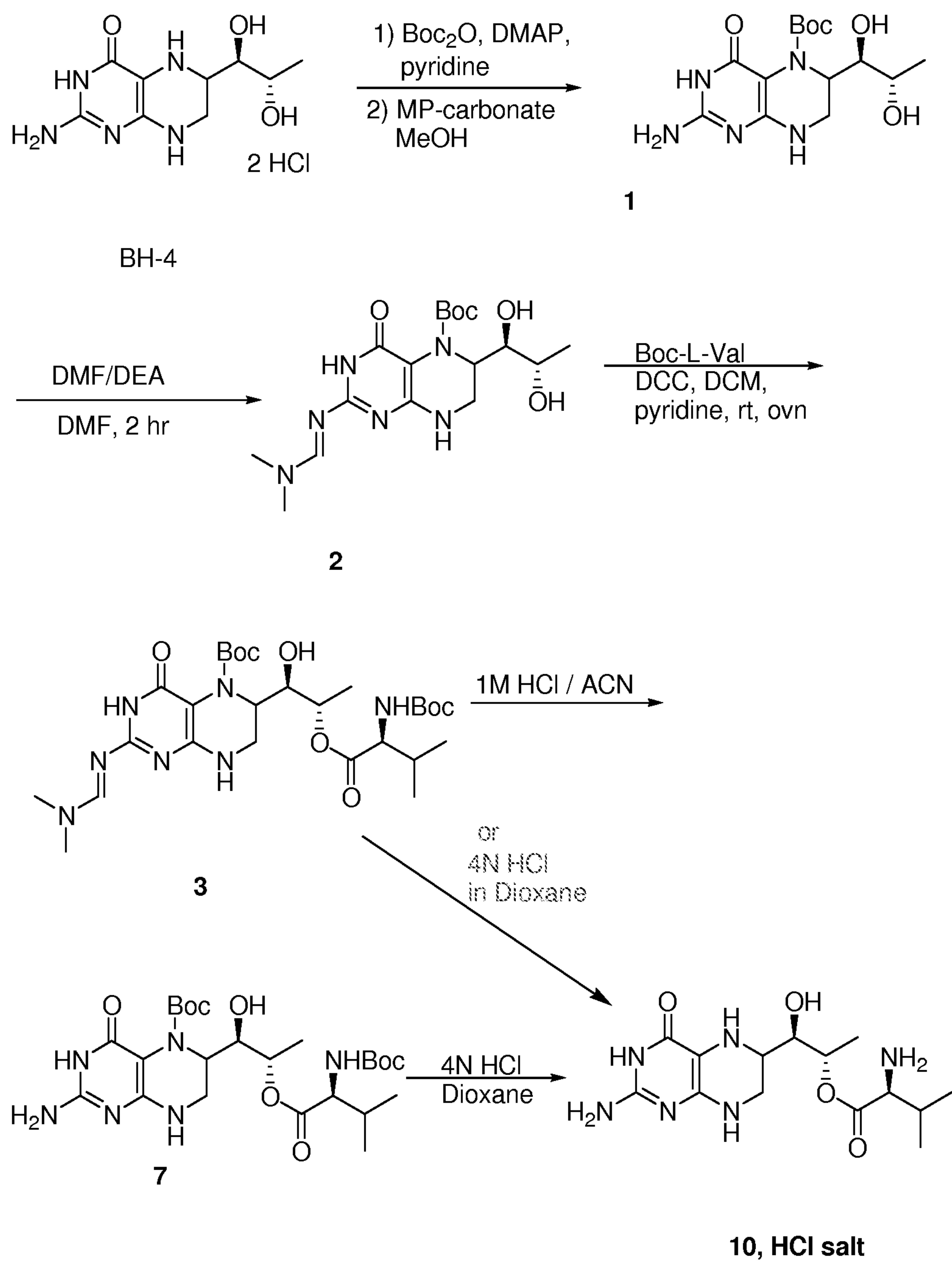
Reaction Scheme (IA')
