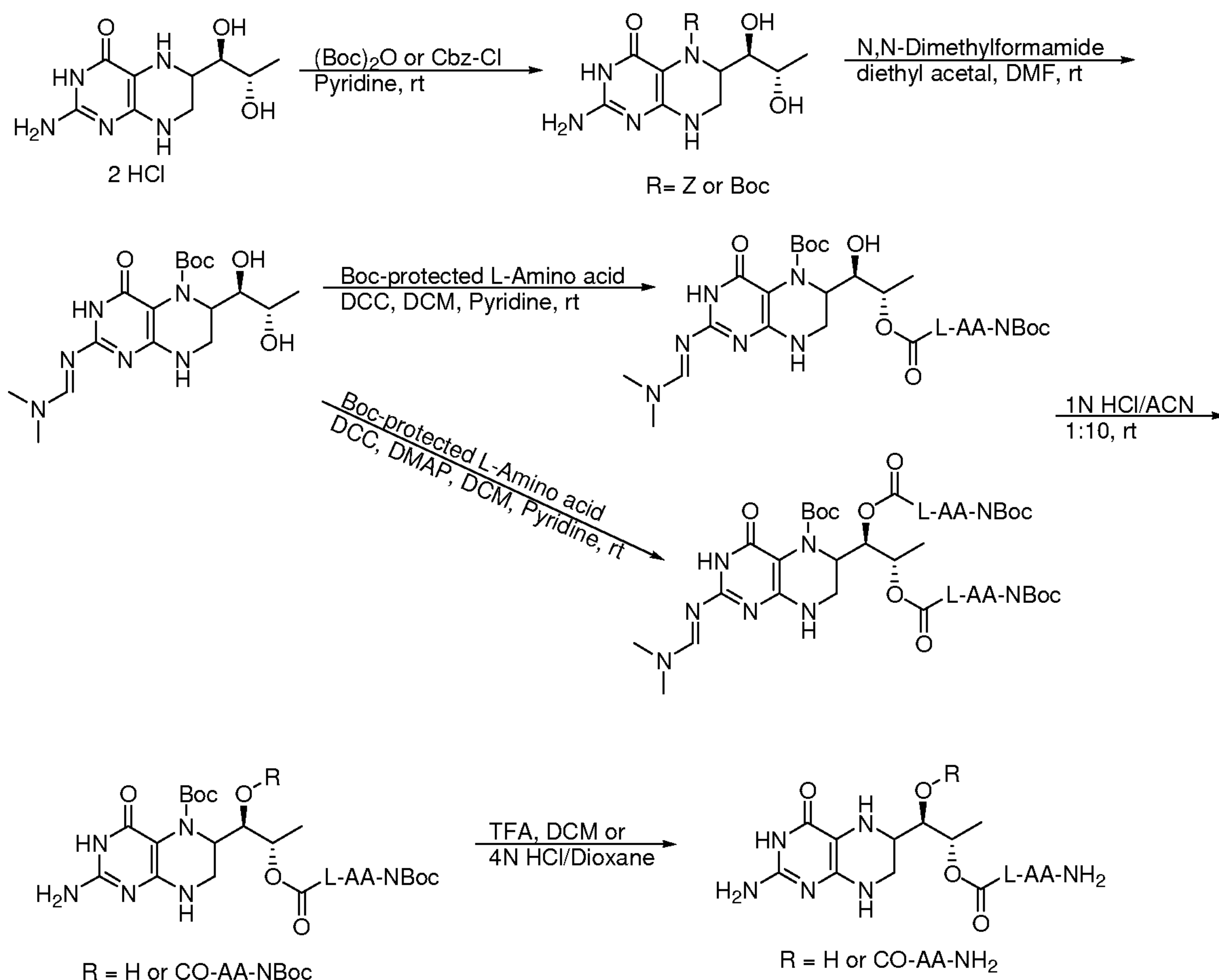
Reaction Scheme (IA)
