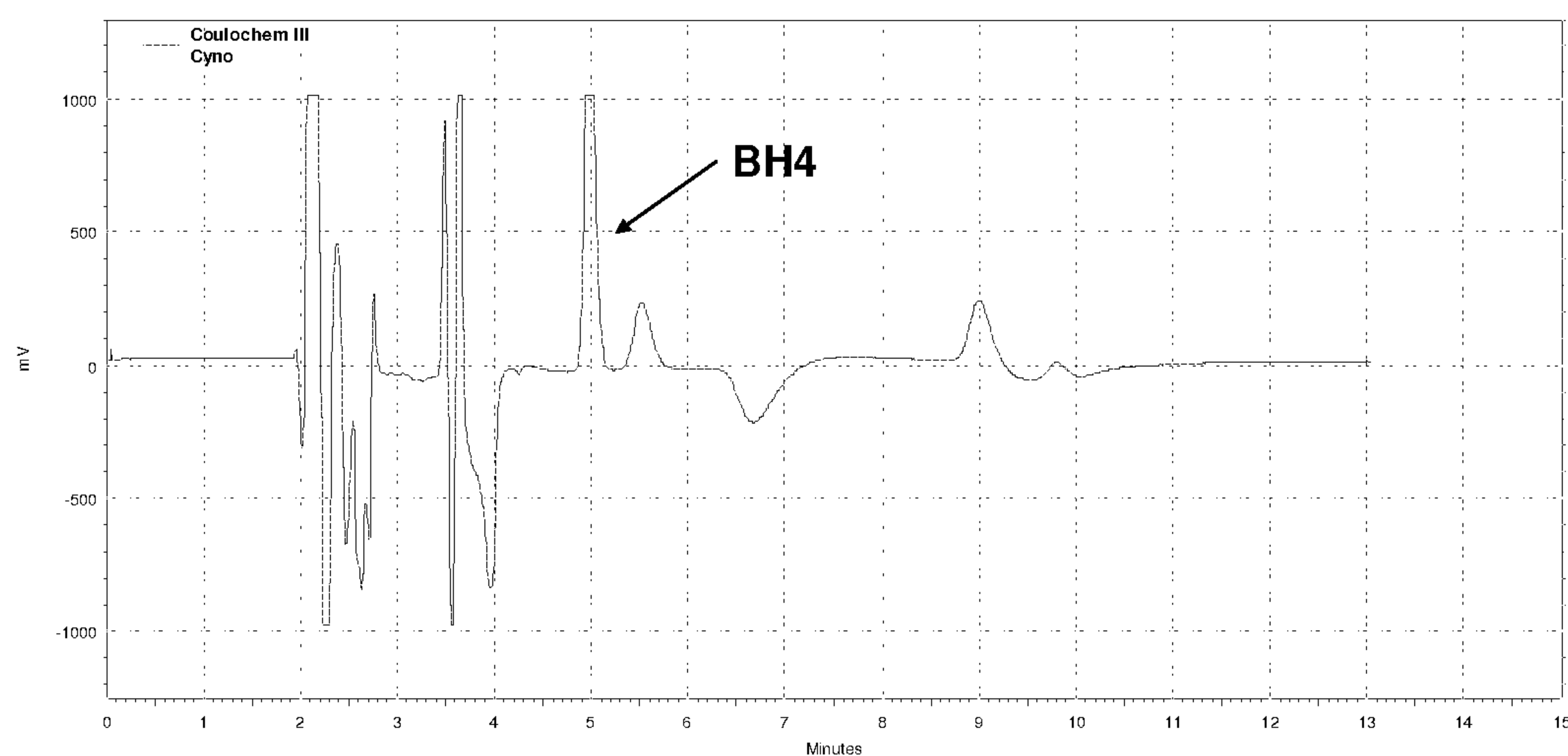
FIGURE 16 - BH4 Chromatogram from Plasma of Cynomolgus Monkeys, 2 hours Post-Administration of the Compound of Example 5 (2% MeOH Mobile Phase)
