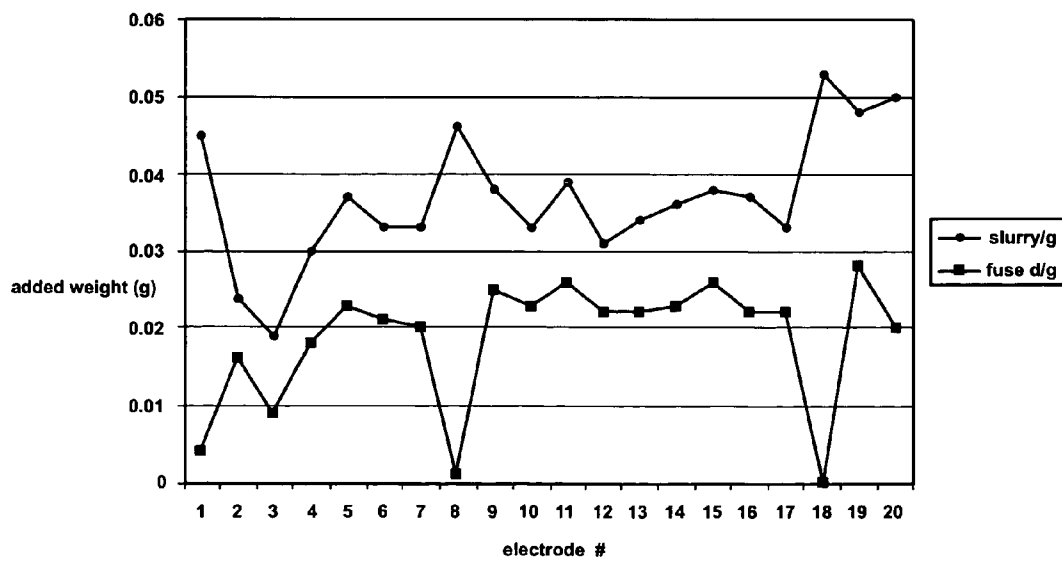
Weight of Ir/Rh/W added to Ni electrode before and after fusing
