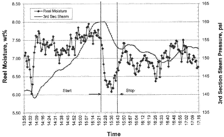
Reel Moisture and 3rd Section Steam Pressure as a Function of Time
