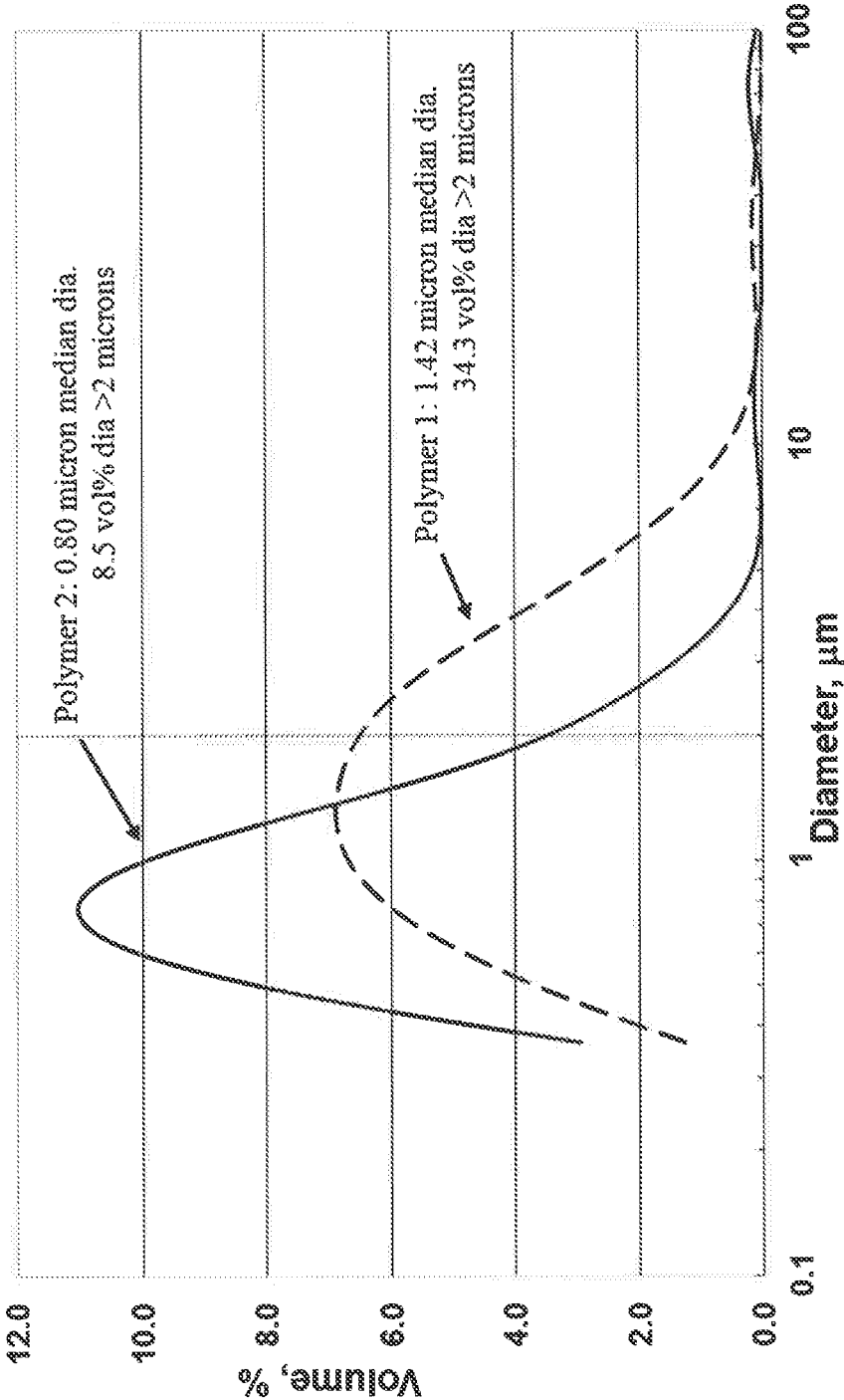
Malvern Particle Size for Emulsification of ASA with Different Polymers
