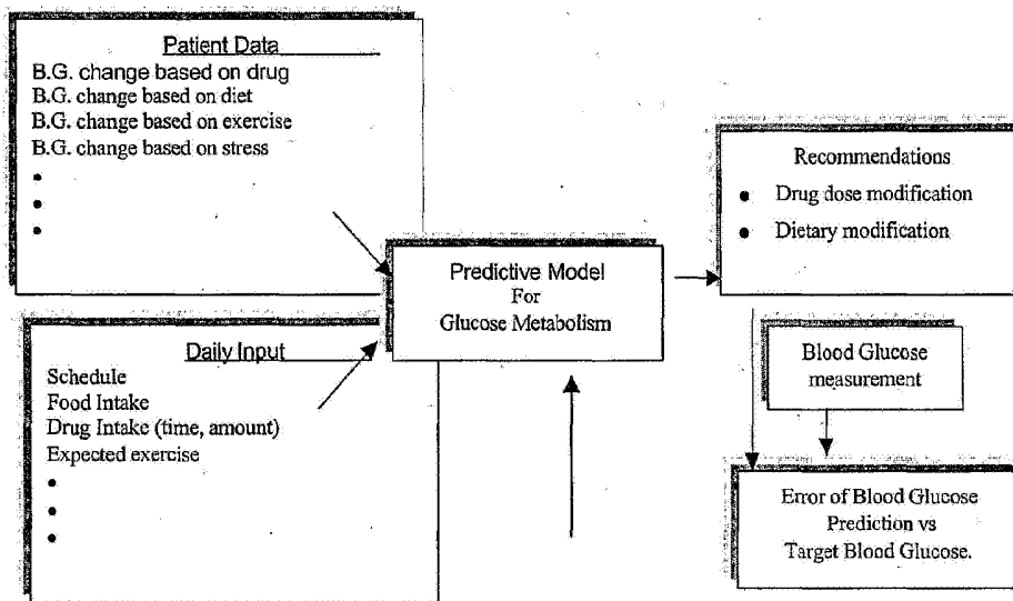
Fig. 26 - shows pictorially how data is typically entered into a Recommender System
