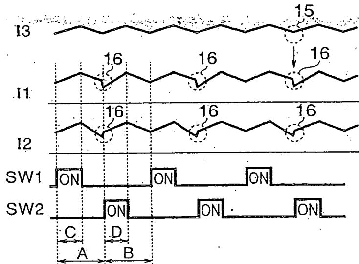
FIG.14 (PRIOR ART)
