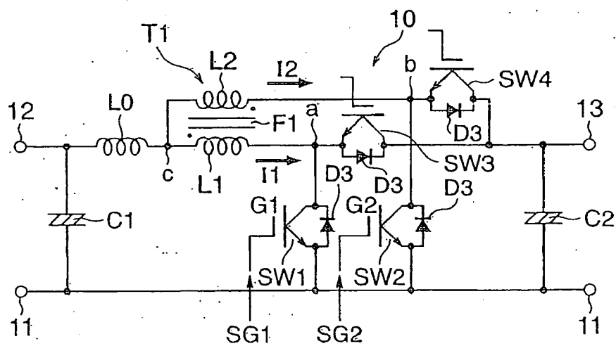
FIG.13 (PRIOR ART)
