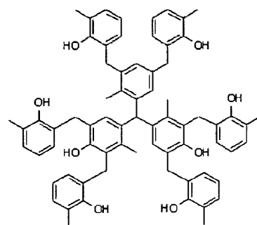
Phenol compound (3)
