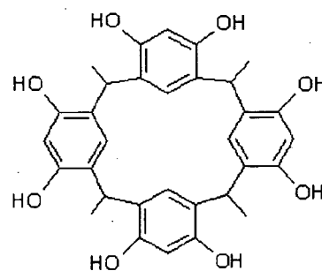
Phenol compound (5)
