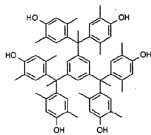
Phenol compound (2)
