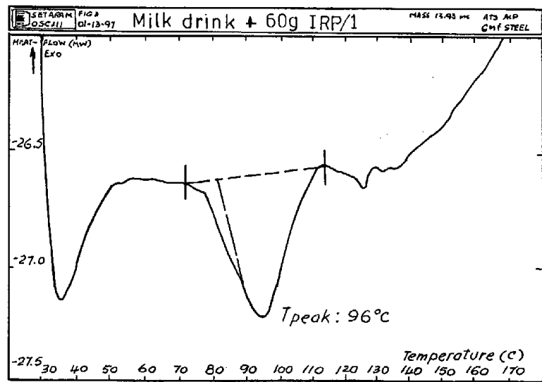
FIG.5 DSC curves of milk drink residues obtained after pancreatin digestion
