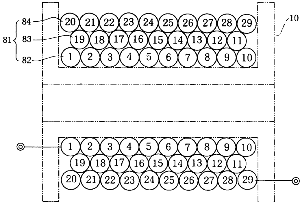
FIG. 11 PRIOR ART
